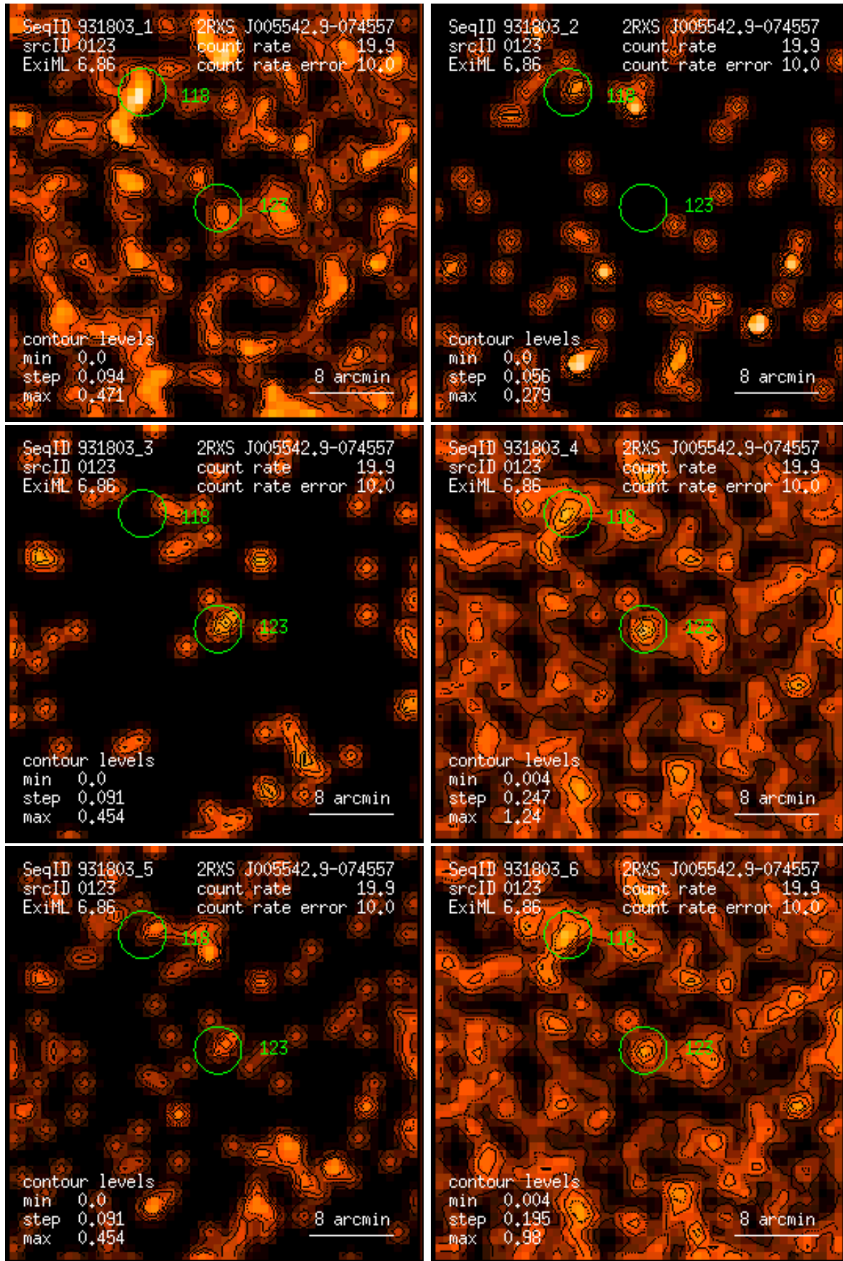
Figure 123: RASS 931803: detection 0123: band rate images, Gaussian filter: (1) PSPC channels 11 – 41, (2) 52 – 90, (3) 91 – 201, (4) 11 – 235, (5) 52 – 201, (6) 11 – 201. Broad band rates in counts/ks. Band rate contour levels in counts/ks/arcmin 2 .
