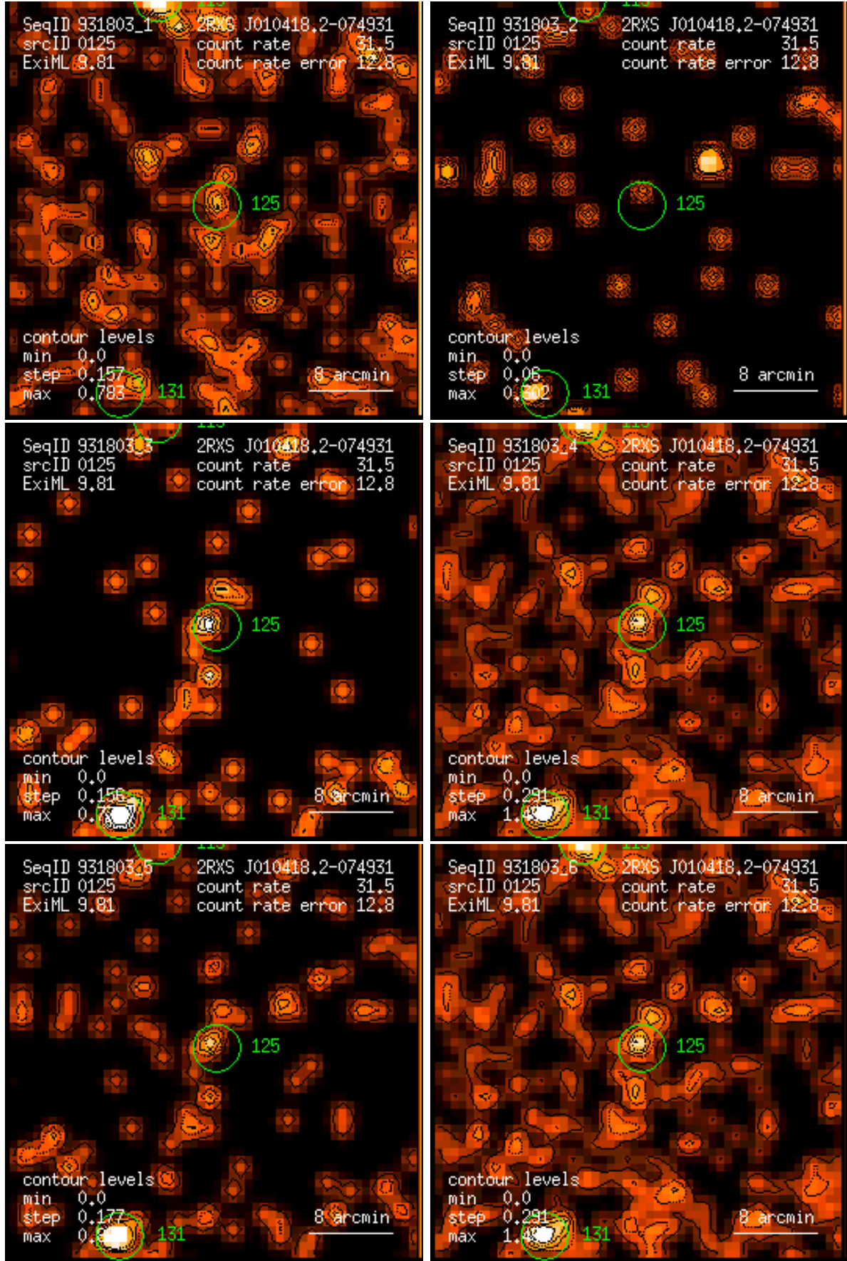
Figure 125: RASS 931803: detection 0125: band rate images, Gaussian filter: (1) PSPC channels 11 – 41, (2) 52 – 90, (3) 91 – 201, (4) 11 – 235, (5) 52 – 201, (6) 11 – 201. Broad band rates in counts/ks. Band rate contour levels in counts/ks/arcmin 2 .
