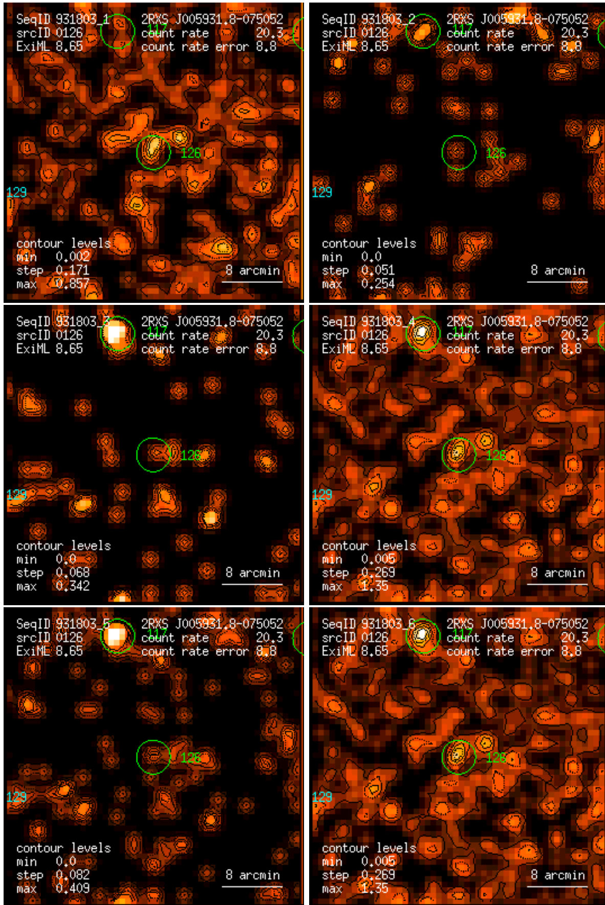
Figure 126: RASS 931803: detection 0126: band rate images, Gaussian filter: (1) PSPC channels 11 – 41, (2) 52 – 90, (3) 91 – 201, (4) 11 – 235, (5) 52 – 201, (6) 11 – 201. Broad band rates in counts/ks. Band rate contour levels in counts/ks/arcmin 2 .
