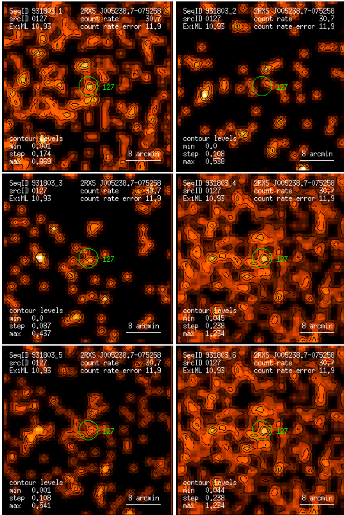
Figure 127: RASS 931803: detection 0127: band rate images, Gaussian filter: (1) PSPC channels 11 – 41, (2) 52 – 90, (3) 91 – 201, (4) 11 – 235, (5) 52 – 201, (6) 11 – 201. Broad band rates in counts/ks. Band rate contour levels in counts/ks/arcmin 2 .
