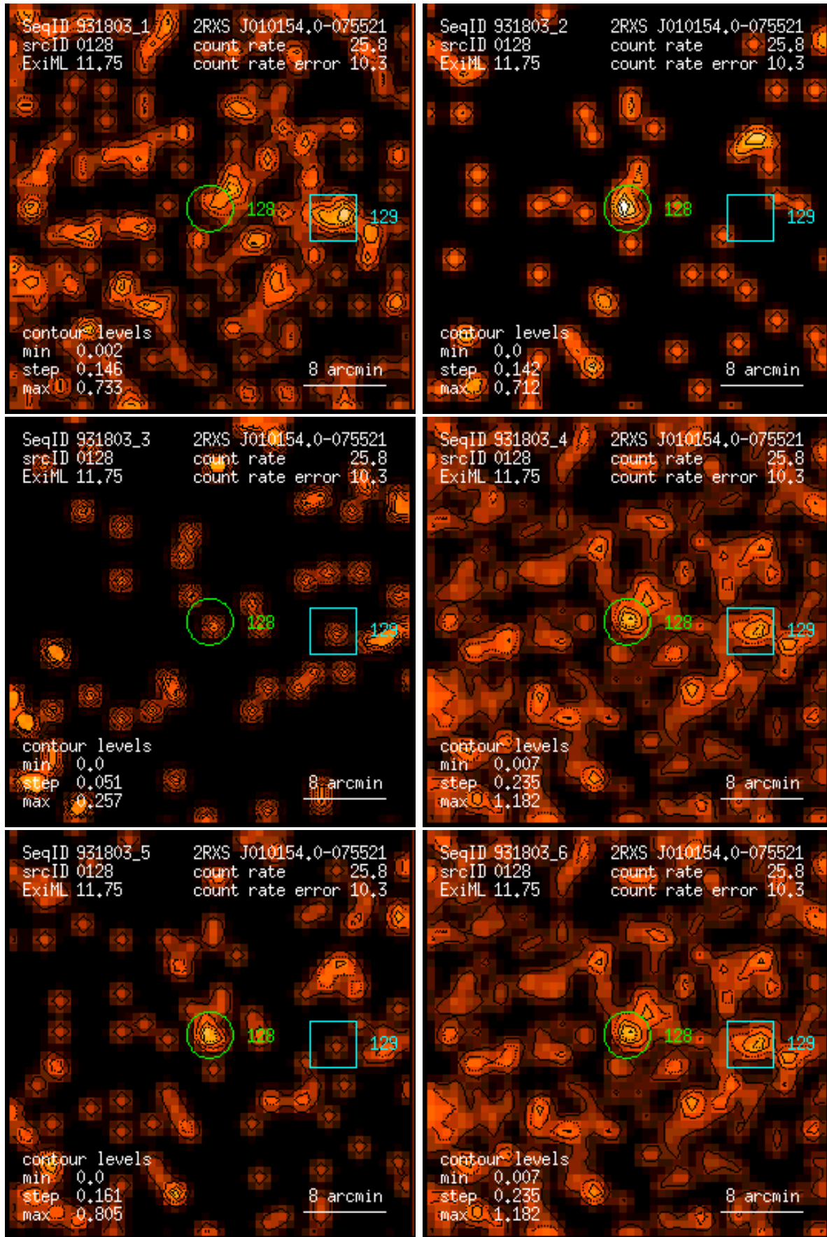
Figure 128: RASS 931803: detection 0128: band rate images, Gaussian filter: (1) PSPC channels 11 – 41, (2) 52 – 90, (3) 91 – 201, (4) 11 – 235, (5) 52 – 201, (6) 11 – 201. Broad band rates in counts/ks. Band rate contour levels in counts/ks/arcmin 2 .
