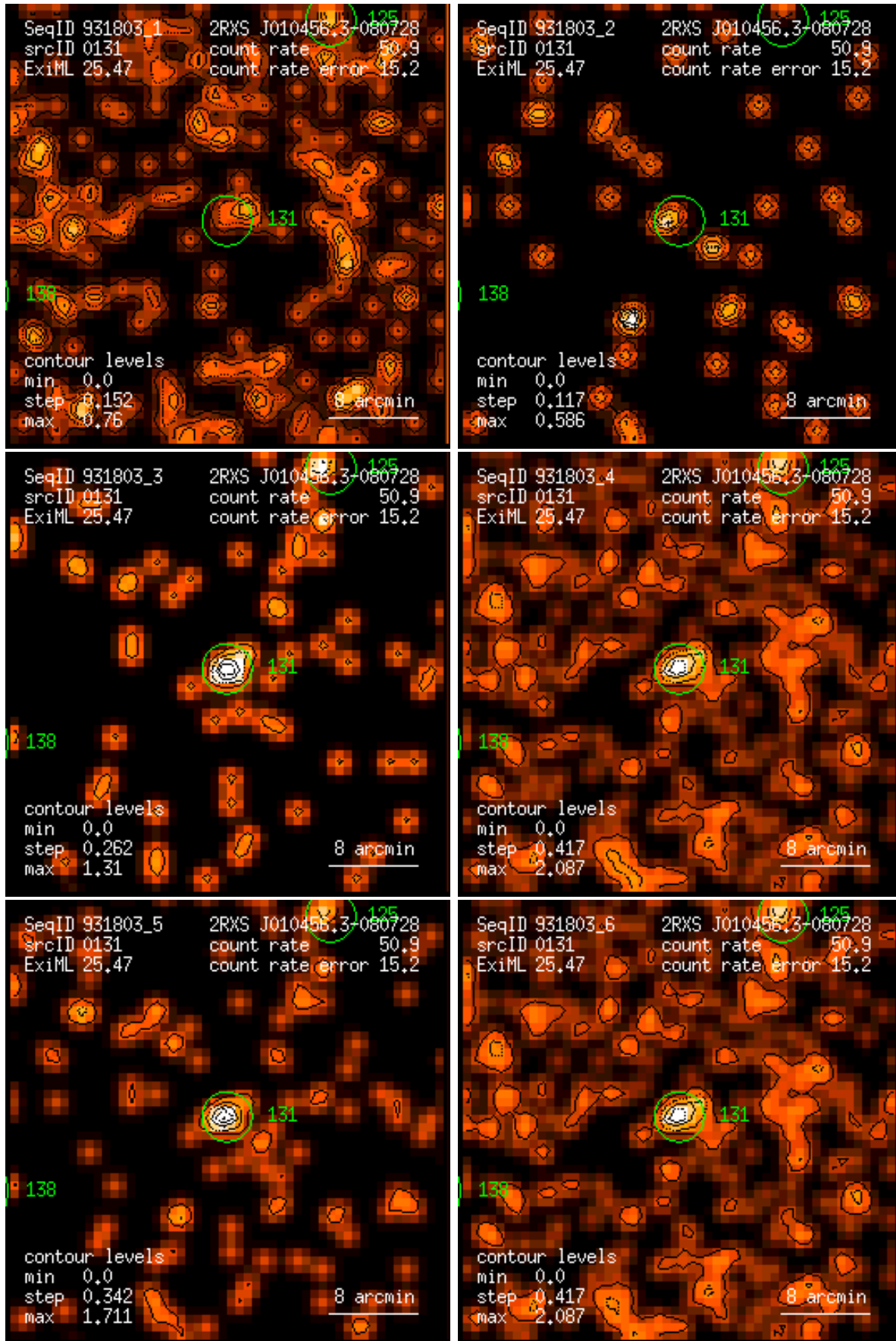
Figure 131: RASS 931803: detection 0131: band rate images, Gaussian filter: (1) PSPC channels 11 – 41, (2) 52 – 90, (3) 91 – 201, (4) 11 – 235, (5) 52 – 201, (6) 11 – 201. Broad band rates in counts/ks. Band rate contour levels in counts/ks/arcmin 2 .
