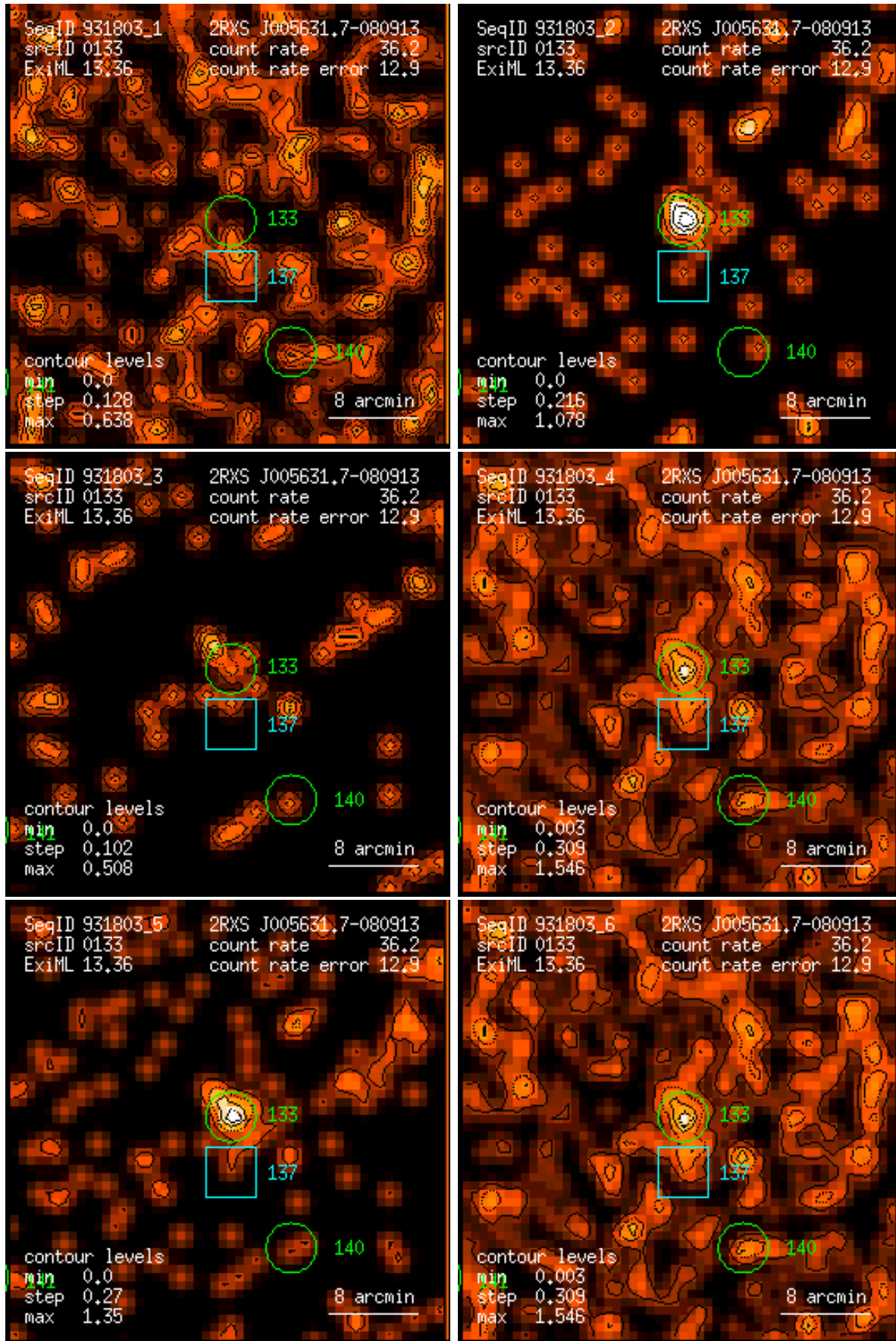
Figure 133: RASS 931803: detection 0133: band rate images, Gaussian filter: (1) PSPC channels 11 – 41, (2) 52 – 90, (3) 91 – 201, (4) 11 – 235, (5) 52 – 201, (6) 11 – 201. Broad band rates in counts/ks. Band rate contour levels in counts/ks/arcmin 2 .
