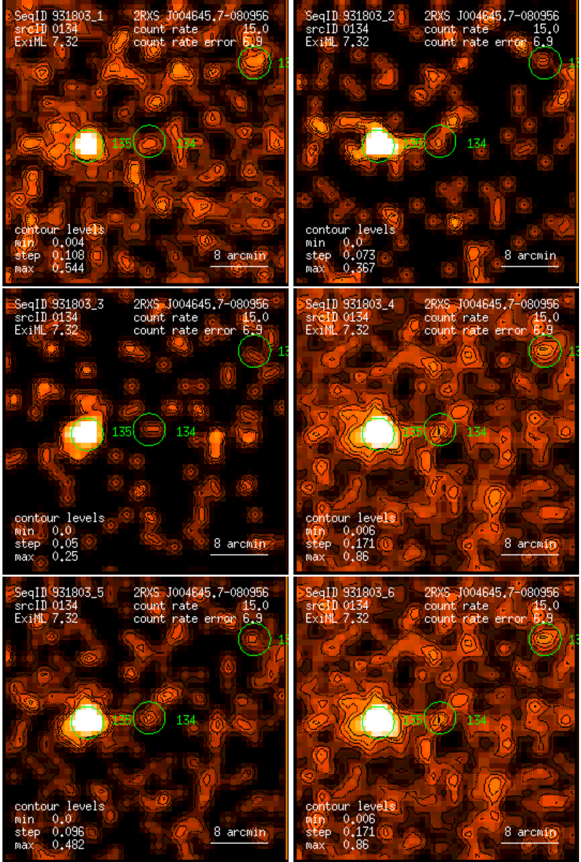
Figure 134: RASS 931803: detection 0134: band rate images, Gaussian filter: (1) PSPC channels 11 – 41, (2) 52 – 90, (3) 91 – 201, (4) 11 – 235, (5) 52 – 201, (6) 11 – 201. Broad band rates in counts/ks. Band rate contour levels in counts/ks/arcmin 2 .
