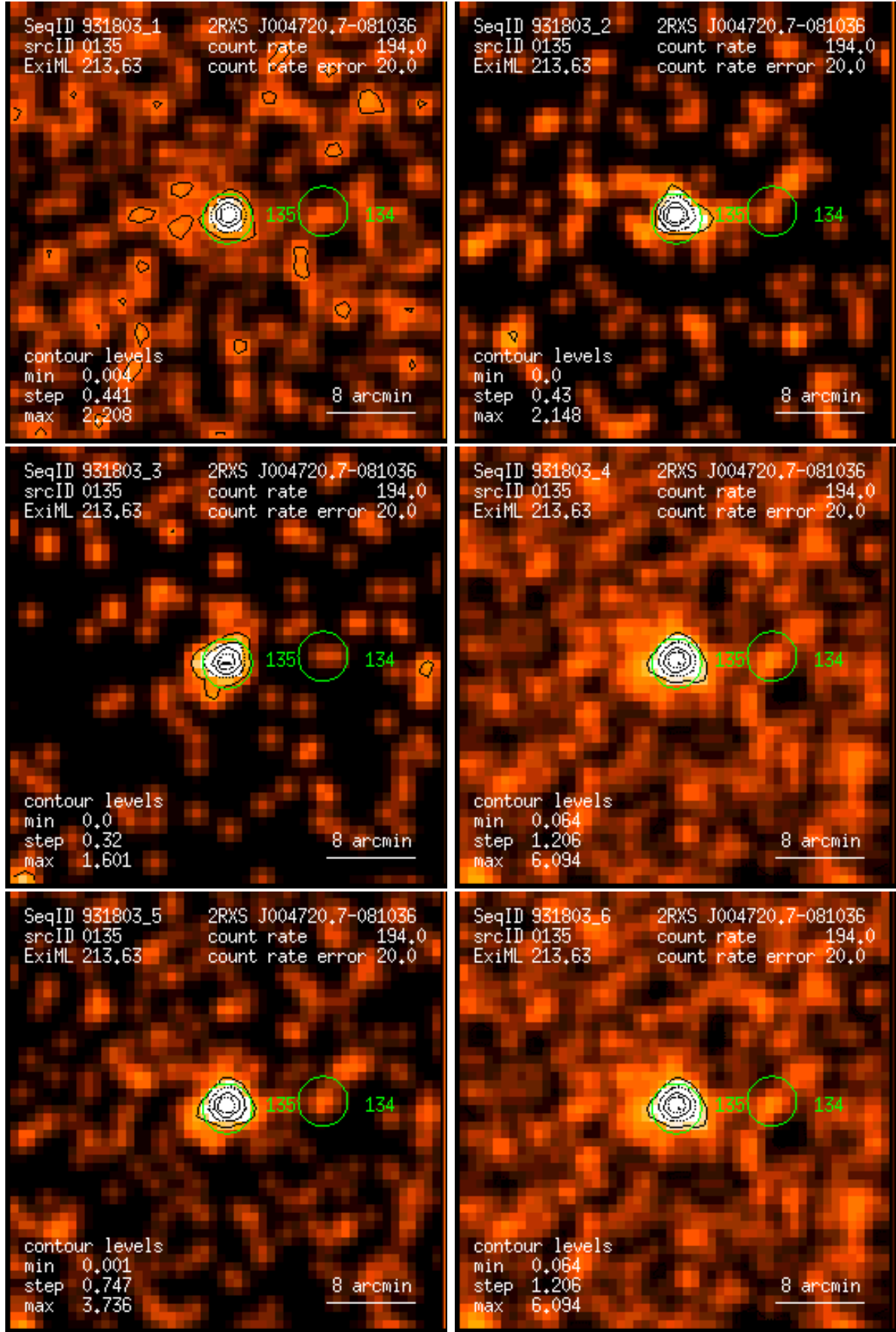
Figure 135: RASS 931803: detection 0135: band rate images, Gaussian filter: (1) PSPC channels 11 – 41, (2) 52 – 90, (3) 91 – 201, (4) 11 – 235, (5) 52 – 201, (6) 11 – 201. Broad band rates in counts/ks. Band rate contour levels in counts/ks/arcmin 2 .
