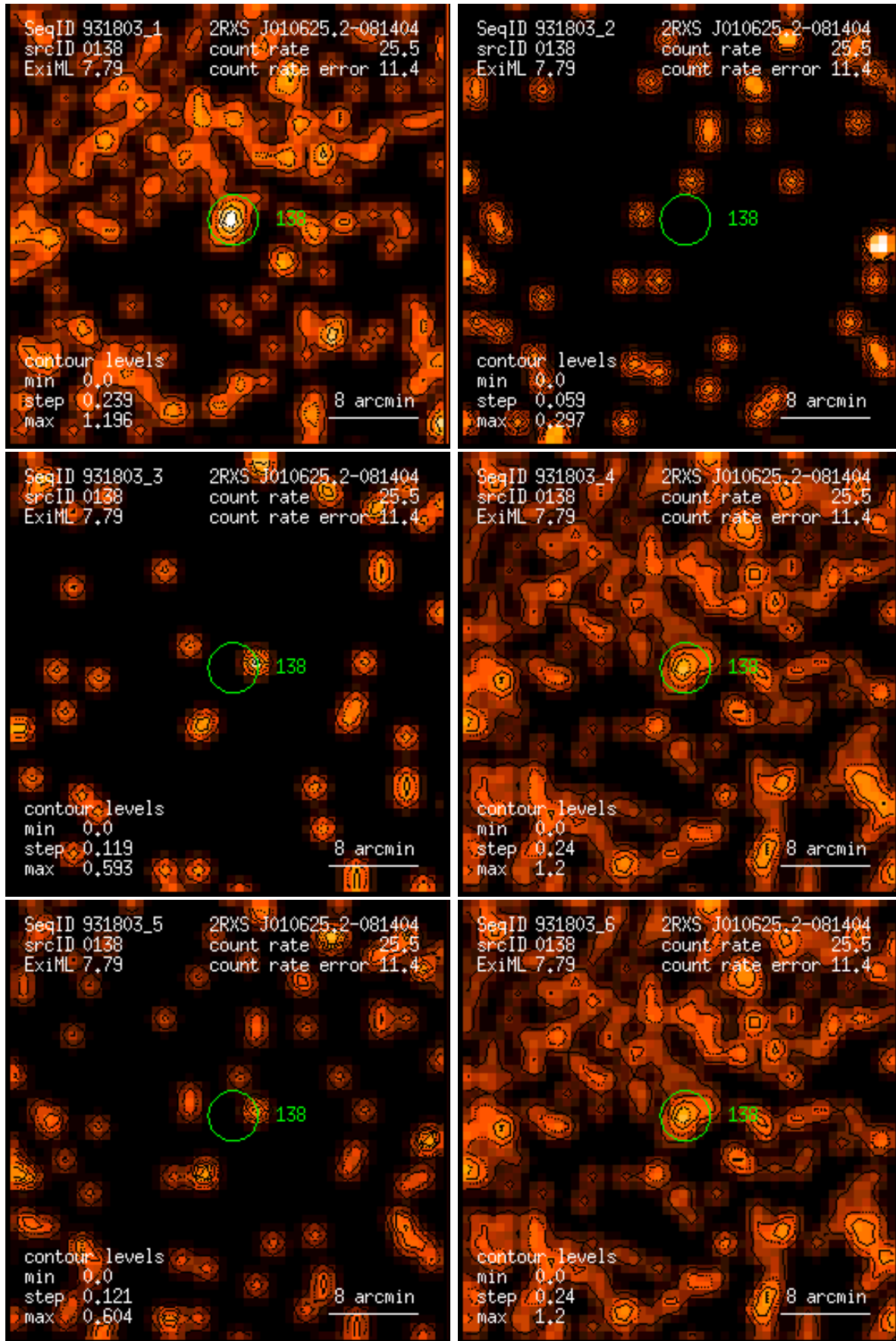
Figure 138: RASS 931803: detection 0138: band rate images, Gaussian filter: (1) PSPC channels 11 – 41, (2) 52 – 90, (3) 91 – 201, (4) 11 – 235, (5) 52 – 201, (6) 11 – 201. Broad band rates in counts/ks. Band rate contour levels in counts/ks/arcmin 2 .
