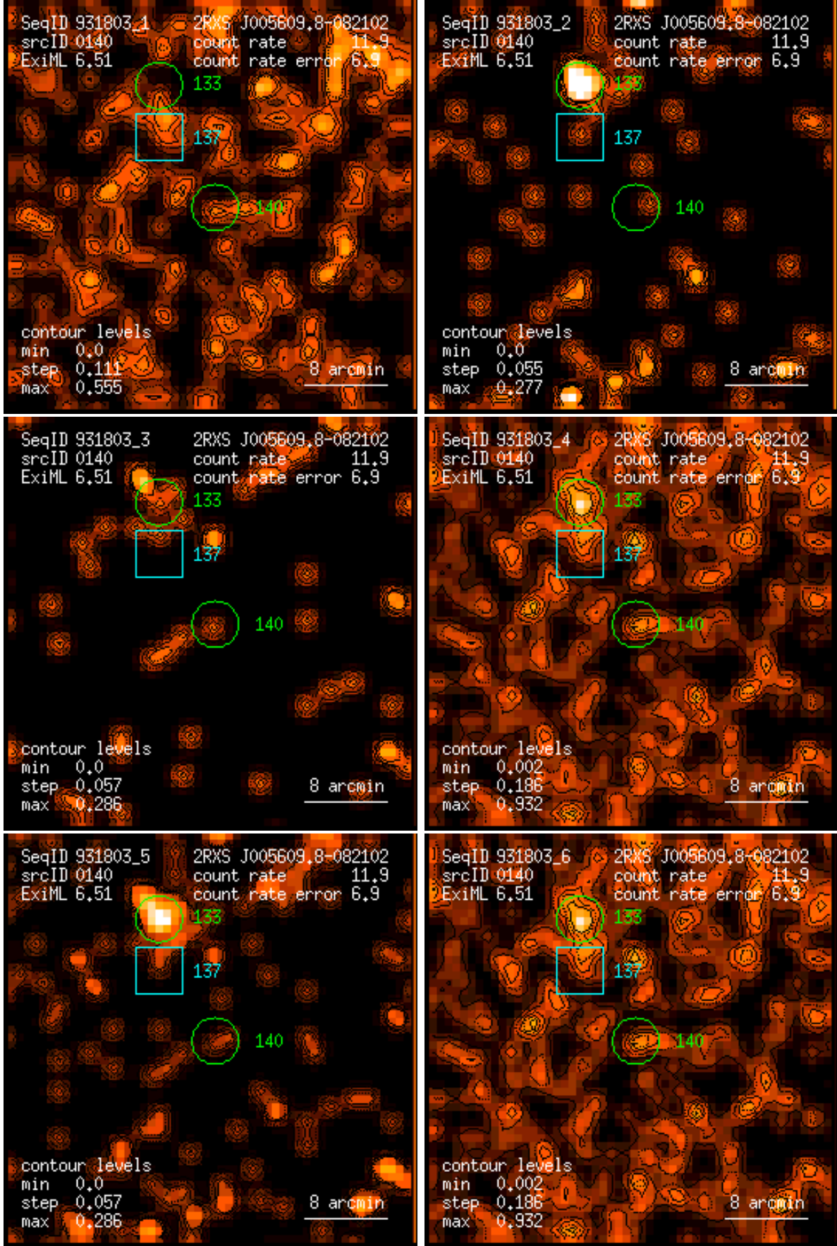
Figure 140: RASS 931803: detection 0140: band rate images, Gaussian filter: (1) PSPC channels 11 – 41, (2) 52 – 90, (3) 91 – 201, (4) 11 – 235, (5) 52 – 201, (6) 11 – 201. Broad band rates in counts/ks. Band rate contour levels in counts/ks/arcmin 2 .
