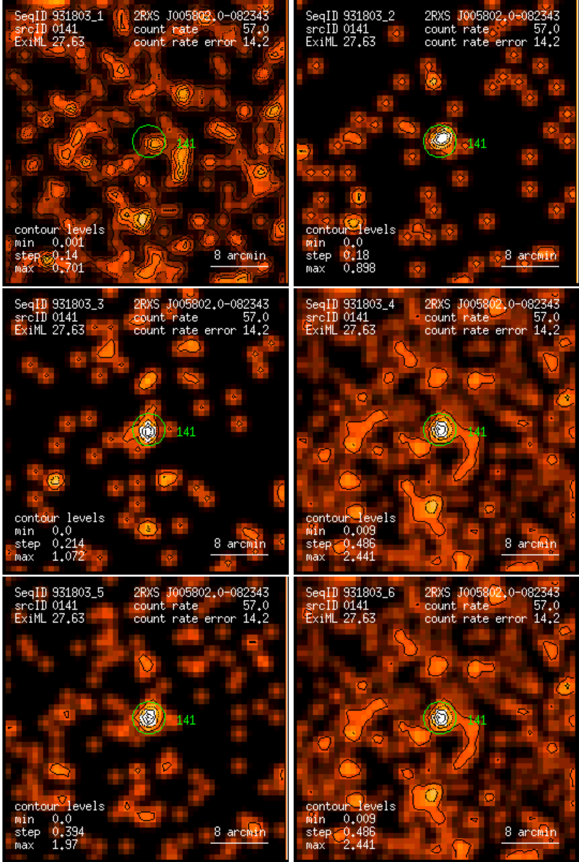
Figure 141: RASS 931803: detection 0141: band rate images, Gaussian filter: (1) PSPC channels 11 – 41, (2) 52 – 90, (3) 91 – 201, (4) 11 – 235, (5) 52 – 201, (6) 11 – 201. Broad band rates in counts/ks. Band rate contour levels in counts/ks/arcmin 2 .
