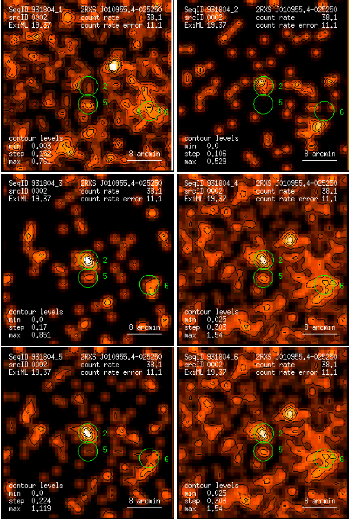
Figure 2: RASS 931804: detection 0002: band rate images, Gaussian filter: (1) PSPC channels 11 – 41, (2) 52 – 90, (3) 91 – 201, (4) 11 – 235, (5) 52 – 201, (6) 11 – 201. Broad band rates in counts/ks. Band rate contour levels in counts/ks/arcmin 2 .
