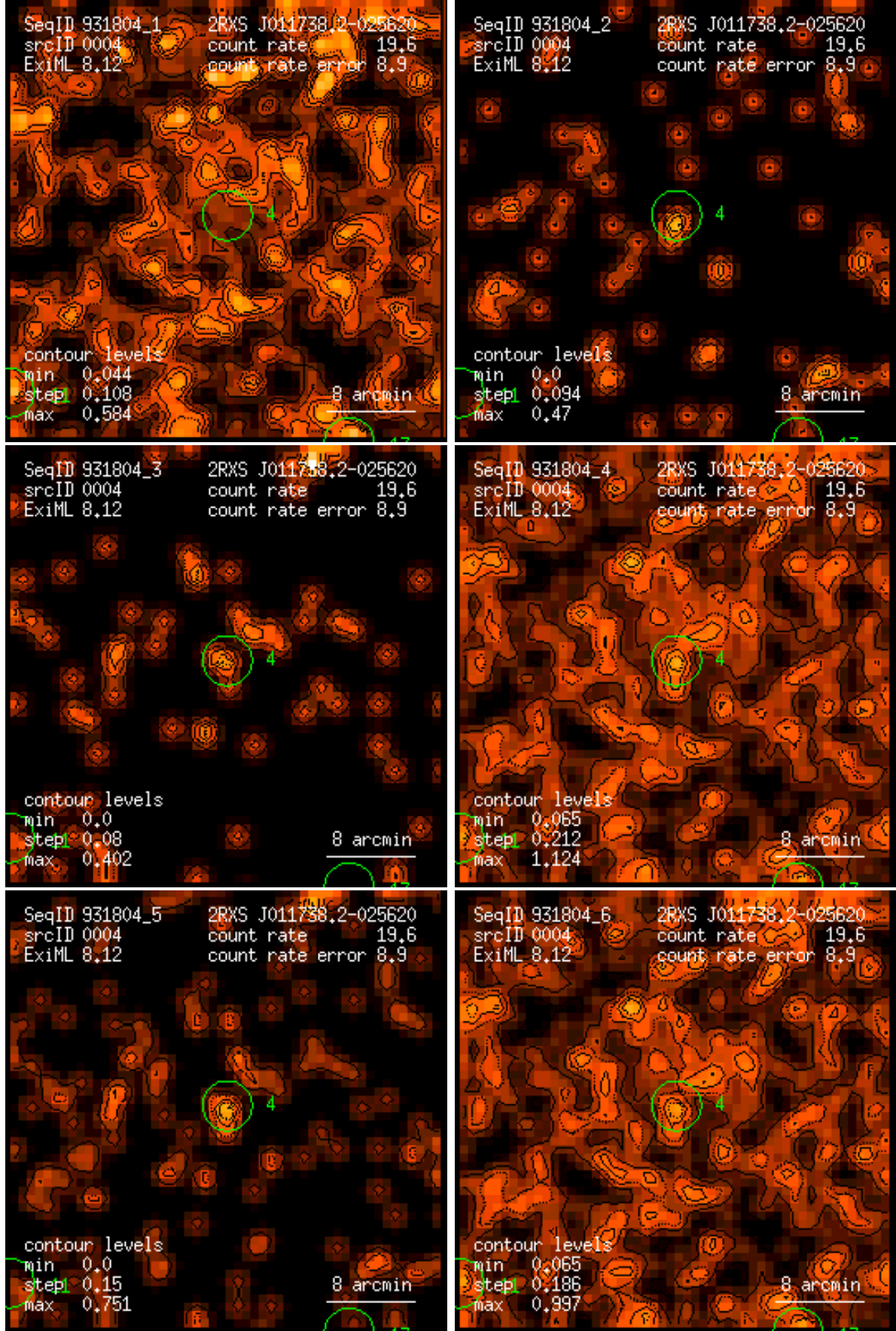
Figure 4: RASS 931804: detection 0004: band rate images, Gaussian filter: (1) PSPC channels 11 – 41, (2) 52 – 90, (3) 91 – 201, (4) 11 – 235, (5) 52 – 201, (6) 11 – 201. Broad band rates in counts/ks. Band rate contour levels in counts/ks/arcmin 2 .
