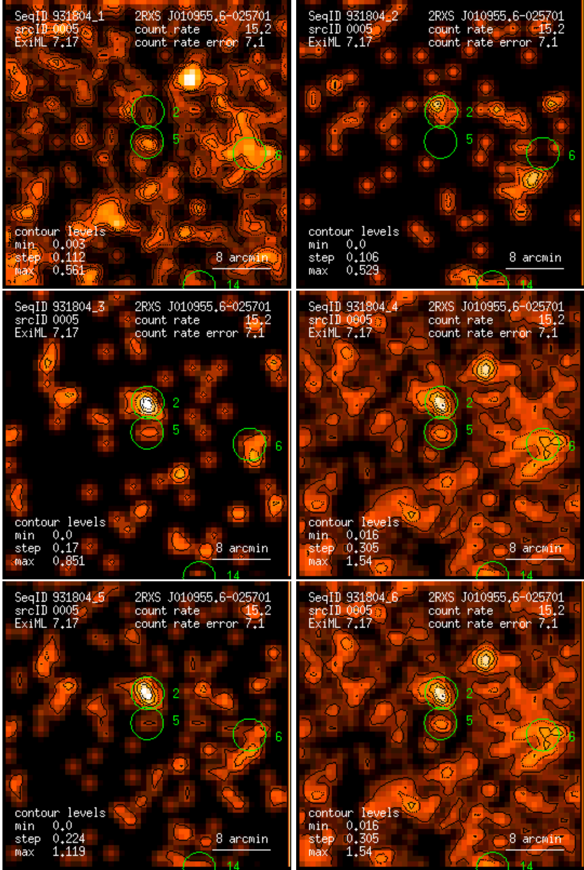
Figure 5: RASS 931804: detection 0005: band rate images, Gaussian filter: (1) PSPC channels 11 – 41, (2) 52 – 90, (3) 91 – 201, (4) 11 – 235, (5) 52 – 201, (6) 11 – 201. Broad band rates in counts/ks. Band rate contour levels in counts/ks/arcmin 2 .
