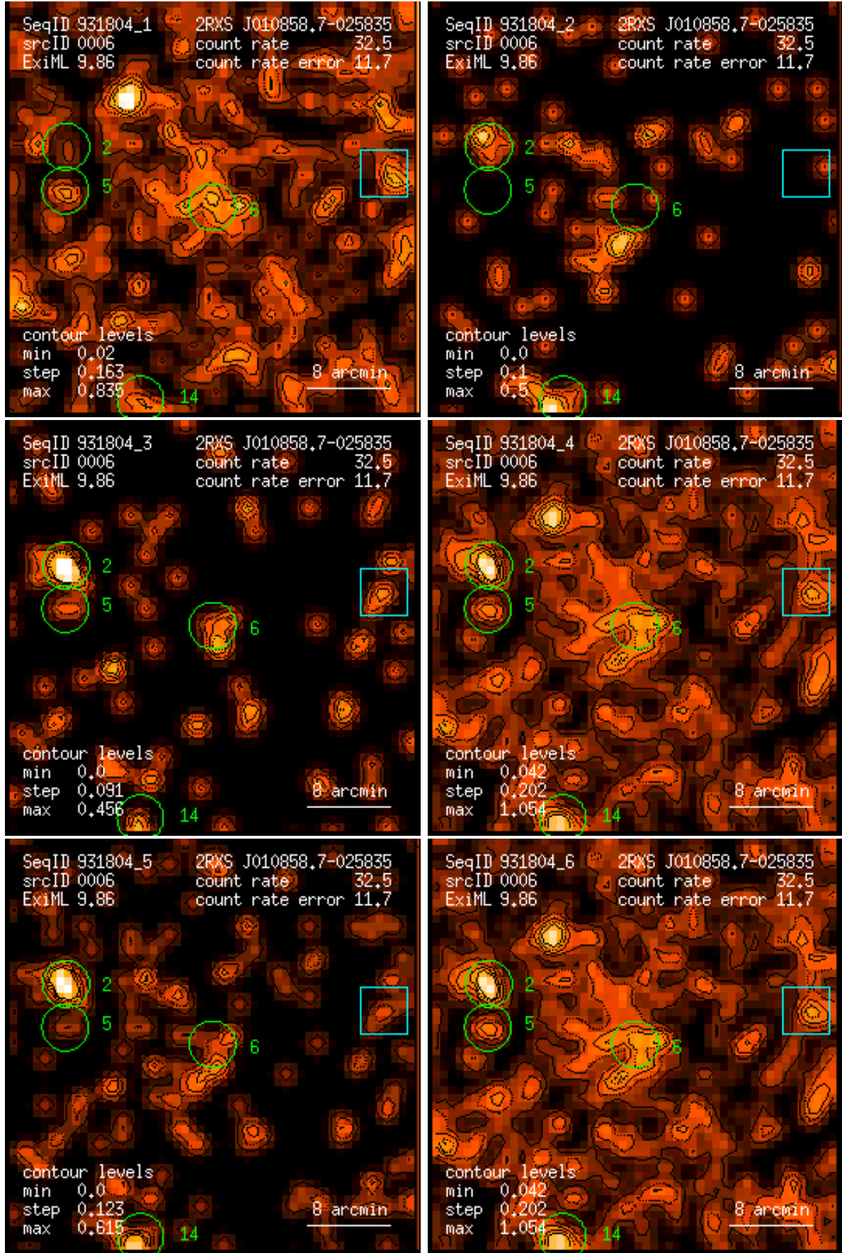
Figure 6: RASS 931804: detection 0006: band rate images, Gaussian filter: (1) PSPC channels 11 – 41, (2) 52 – 90, (3) 91 – 201, (4) 11 – 235, (5) 52 – 201, (6) 11 – 201. Broad band rates in counts/ks. Band rate contour levels in counts/ks/arcmin 2 .
