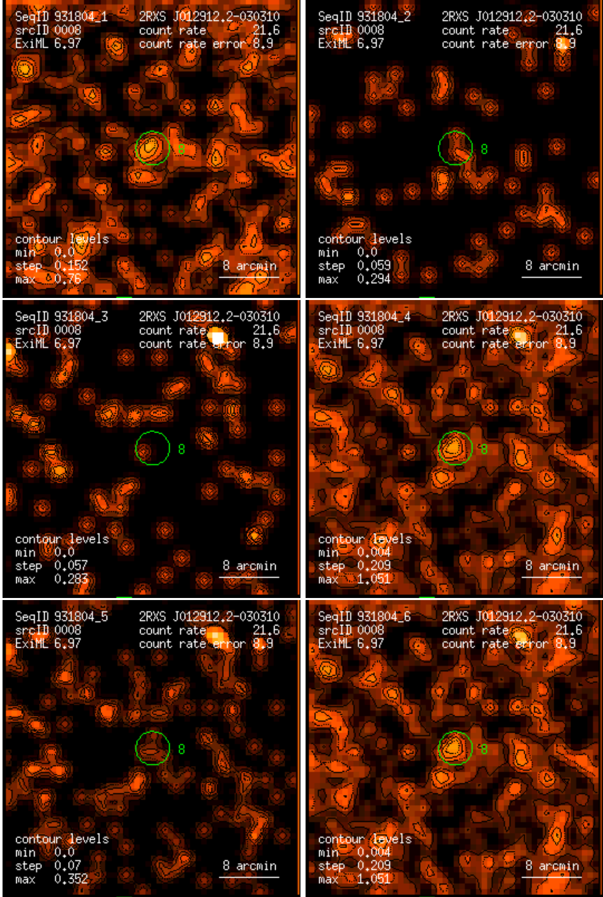
Figure 8: RASS 931804: detection 0008: band rate images, Gaussian filter: (1) PSPC channels 11 – 41, (2) 52 – 90, (3) 91 – 201, (4) 11 – 235, (5) 52 – 201, (6) 11 – 201. Broad band rates in counts/ks. Band rate contour levels in counts/ks/arcmin 2 .
