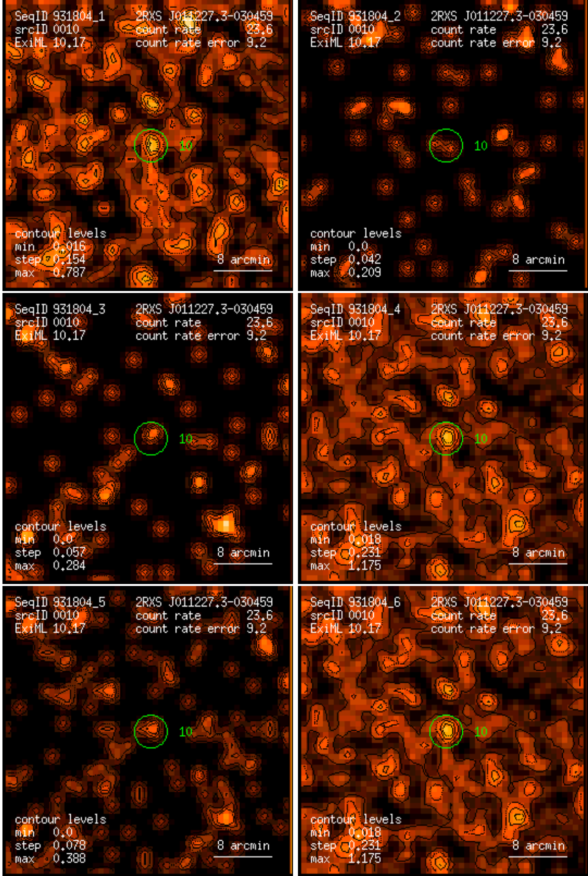
Figure 10: RASS 931804: detection 0010: band rate images, Gaussian filter: (1) PSPC channels 11 – 41, (2) 52 – 90, (3) 91 – 201, (4) 11 – 235, (5) 52 – 201, (6) 11 – 201. Broad band rates in counts/ks. Band rate contour levels in counts/ks/arcmin 2 .
