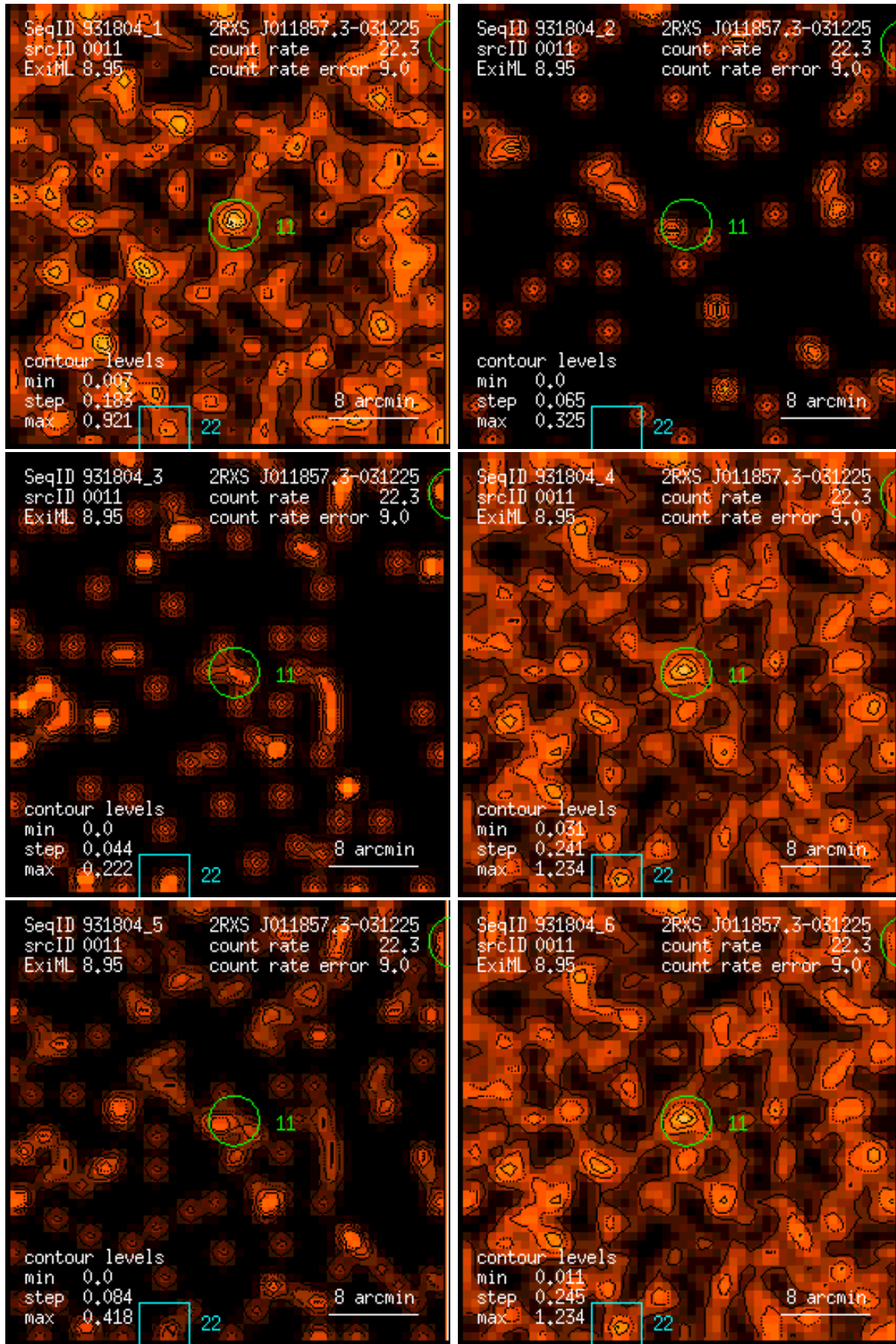
Figure 11: RASS 931804: detection 0011: band rate images, Gaussian filter: (1) PSPC channels 11 – 41, (2) 52 – 90, (3) 91 – 201, (4) 11 – 235, (5) 52 – 201, (6) 11 – 201. Broad band rates in counts/ks. Band rate contour levels in counts/ks/arcmin 2 .
