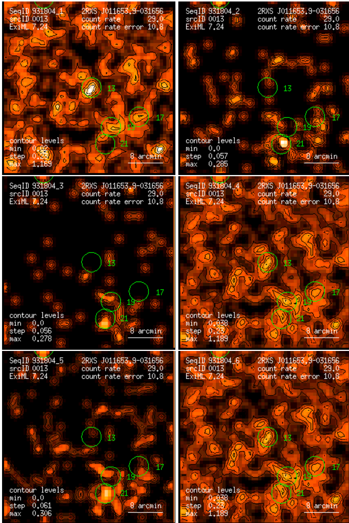
Figure 13: RASS 931804: detection 0013: band rate images, Gaussian filter: (1) PSPC channels 11 – 41, (2) 52 – 90, (3) 91 – 201, (4) 11 – 235, (5) 52 – 201, (6) 11 – 201. Broad band rates in counts/ks. Band rate contour levels in counts/ks/arcmin 2 .
