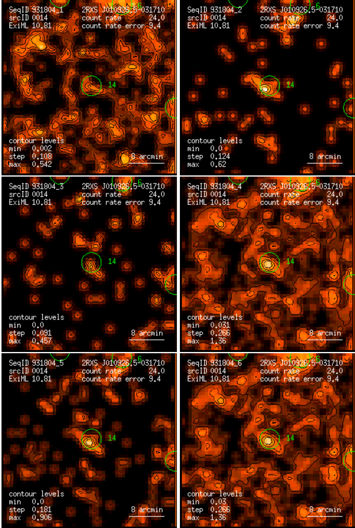
Figure 14: RASS 931804: detection 0014: band rate images, Gaussian filter: (1) PSPC channels 11 – 41, (2) 52 – 90, (3) 91 – 201, (4) 11 – 235, (5) 52 – 201, (6) 11 – 201. Broad band rates in counts/ks. Band rate contour levels in counts/ks/arcmin 2 .
