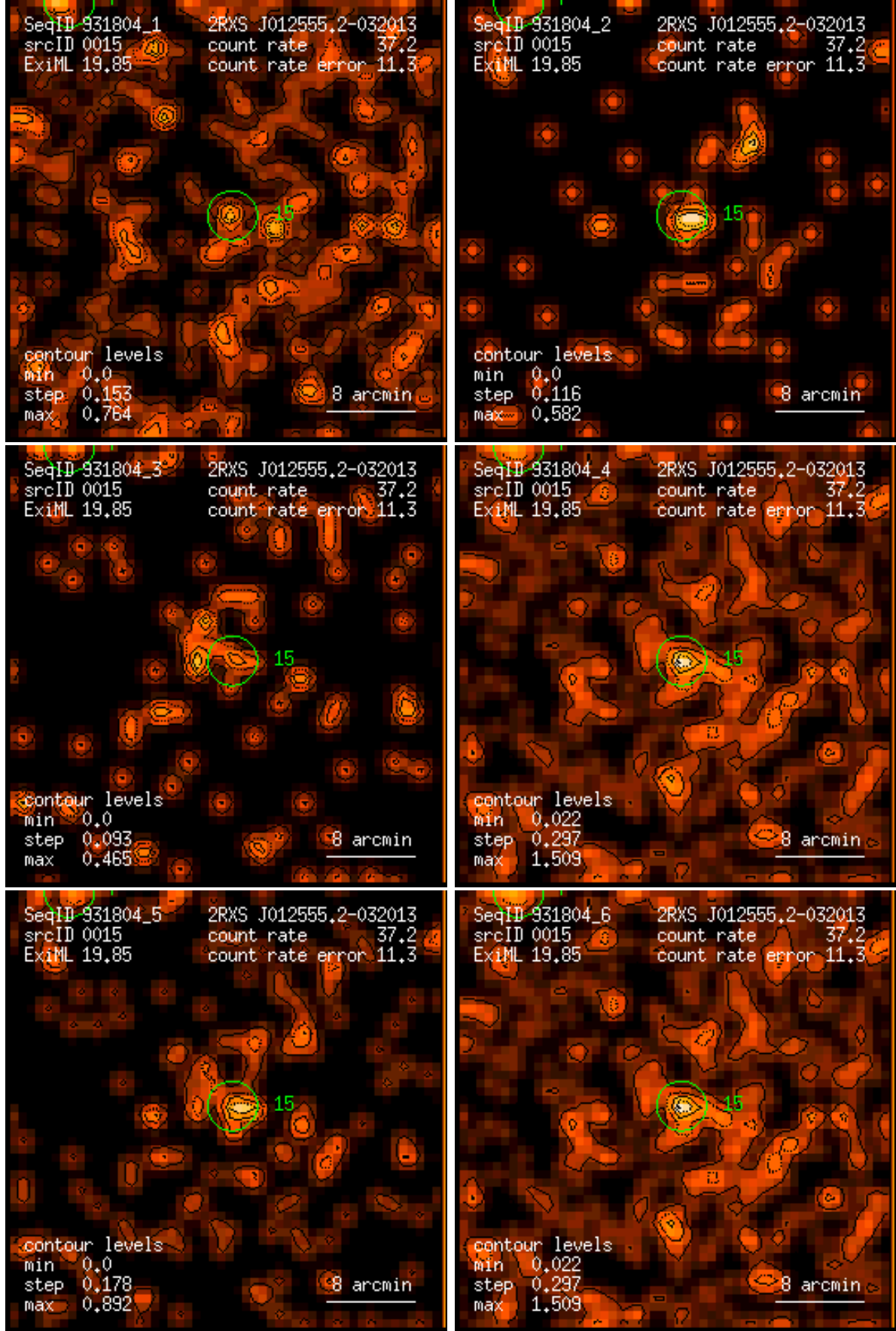
Figure 15: RASS 931804: detection 0015: band rate images, Gaussian filter: (1) PSPC channels 11 – 41, (2) 52 – 90, (3) 91 – 201, (4) 11 – 235, (5) 52 – 201, (6) 11 – 201. Broad band rates in counts/ks. Band rate contour levels in counts/ks/arcmin 2 .
