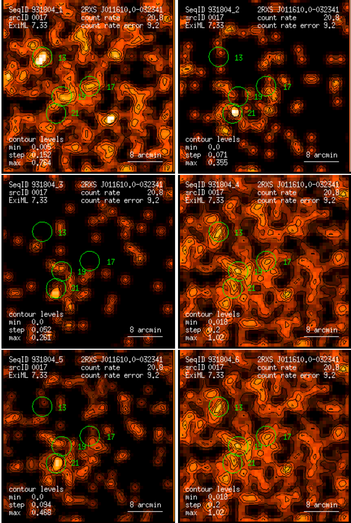
Figure 17: RASS 931804: detection 0017: band rate images, Gaussian filter: (1) PSPC channels 11 – 41, (2) 52 – 90, (3) 91 – 201, (4) 11 – 235, (5) 52 – 201, (6) 11 – 201. Broad band rates in counts/ks. Band rate contour levels in counts/ks/arcmin 2 .
