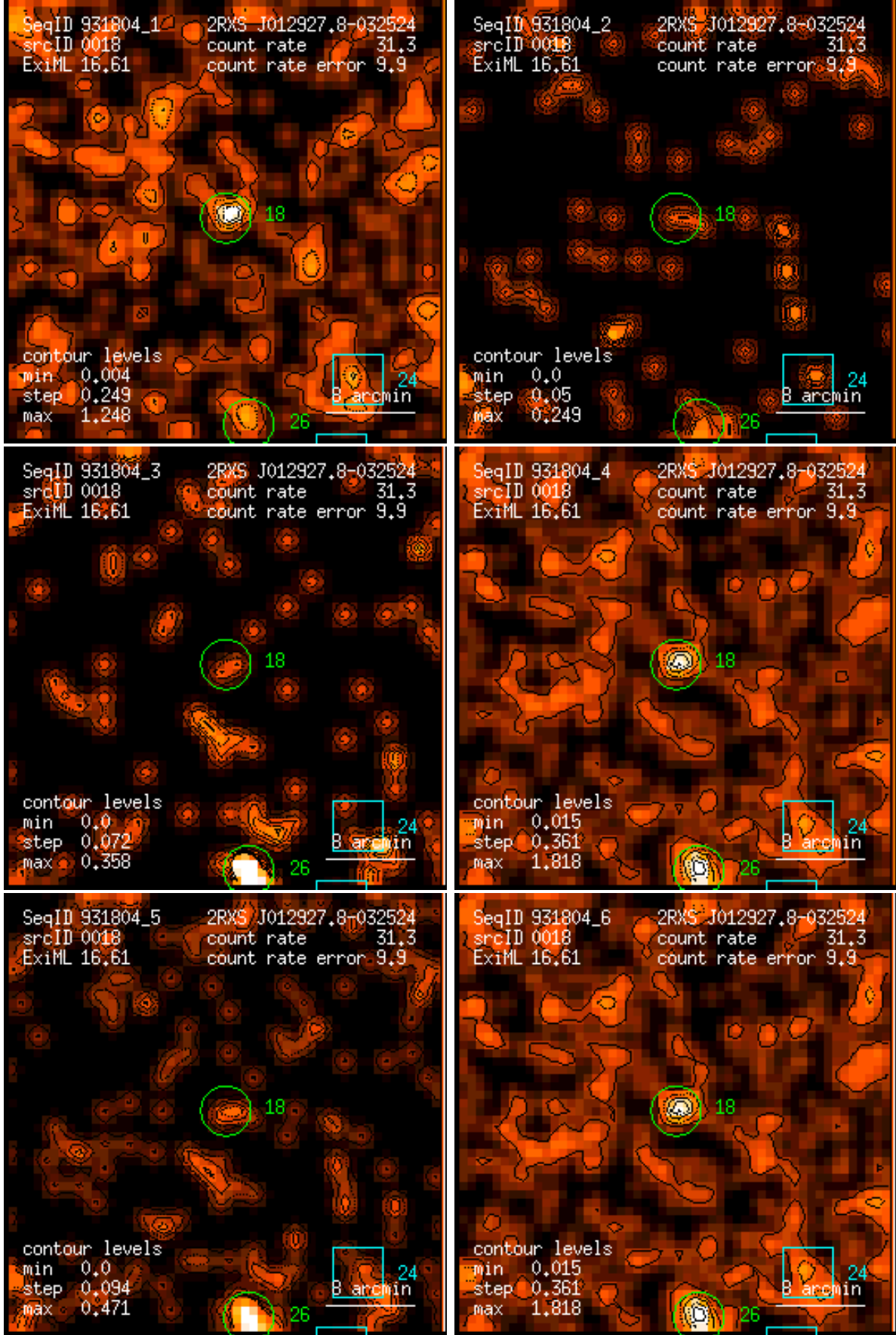
Figure 18: RASS 931804: detection 0018: band rate images, Gaussian filter: (1) PSPC channels 11 – 41, (2) 52 – 90, (3) 91 – 201, (4) 11 – 235, (5) 52 – 201, (6) 11 – 201. Broad band rates in counts/ks. Band rate contour levels in counts/ks/arcmin 2 .
