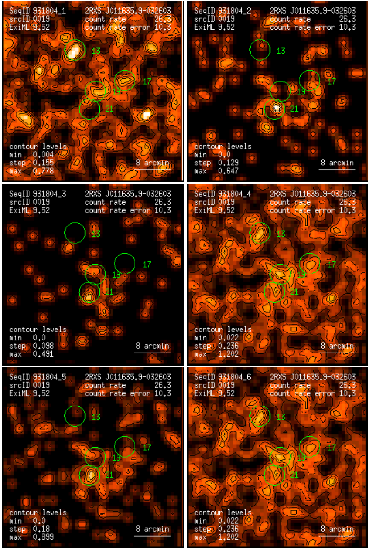
Figure 19: RASS 931804: detection 0019: band rate images, Gaussian filter: (1) PSPC channels 11 – 41, (2) 52 – 90, (3) 91 – 201, (4) 11 – 235, (5) 52 – 201, (6) 11 – 201. Broad band rates in counts/ks. Band rate contour levels in counts/ks/arcmin 2 .
