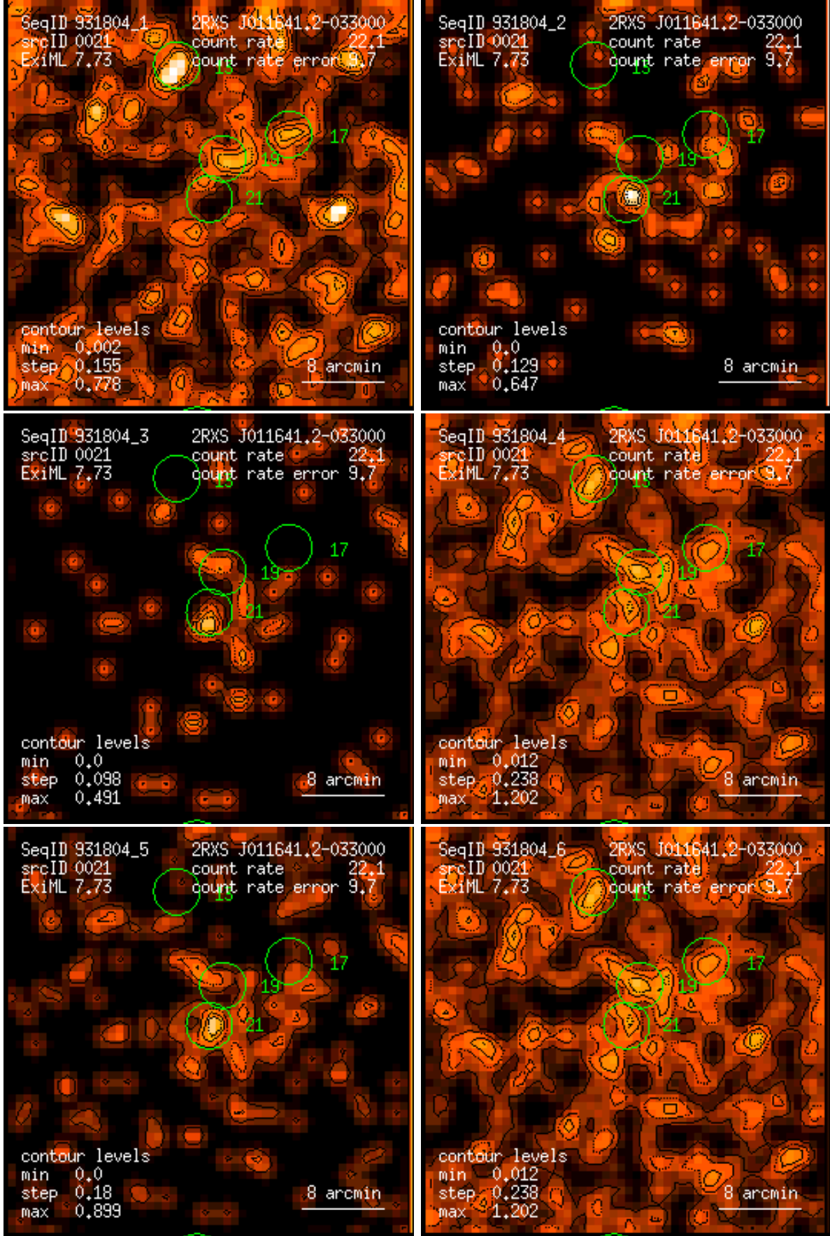
Figure 21: RASS 931804: detection 0021: band rate images, Gaussian filter: (1) PSPC channels 11 – 41, (2) 52 – 90, (3) 91 – 201, (4) 11 – 235, (5) 52 – 201, (6) 11 – 201. Broad band rates in counts/ks. Band rate contour levels in counts/ks/arcmin 2 .
