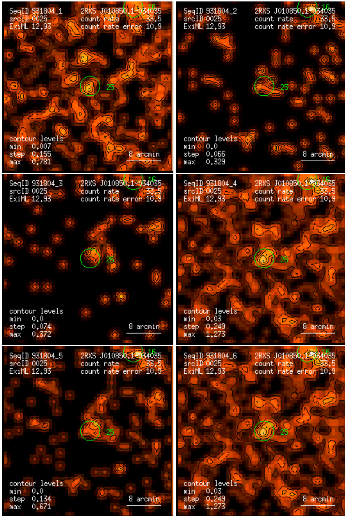
Figure 25: RASS 931804: detection 0025: band rate images, Gaussian filter: (1) PSPC channels 11 – 41, (2) 52 – 90, (3) 91 – 201, (4) 11 – 235, (5) 52 – 201, (6) 11 – 201. Broad band rates in counts/ks. Band rate contour levels in counts/ks/arcmin 2 .
