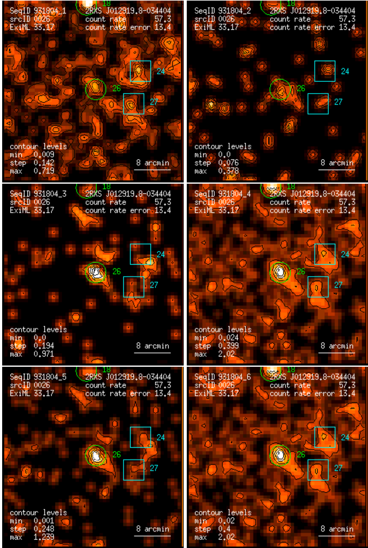
Figure 26: RASS 931804: detection 0026: band rate images, Gaussian filter: (1) PSPC channels 11 – 41, (2) 52 – 90, (3) 91 – 201, (4) 11 – 235, (5) 52 – 201, (6) 11 – 201. Broad band rates in counts/ks. Band rate contour levels in counts/ks/arcmin 2 .
