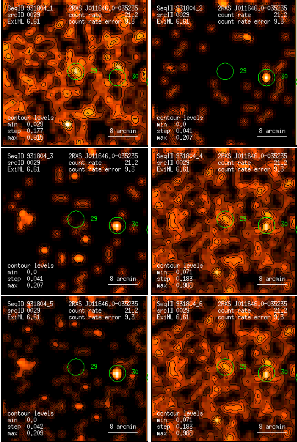
Figure 29: RASS 931804: detection 0029: band rate images, Gaussian filter: (1) PSPC channels 11 – 41, (2) 52 – 90, (3) 91 – 201, (4) 11 – 235, (5) 52 – 201, (6) 11 – 201. Broad band rates in counts/ks. Band rate contour levels in counts/ks/arcmin 2 .
