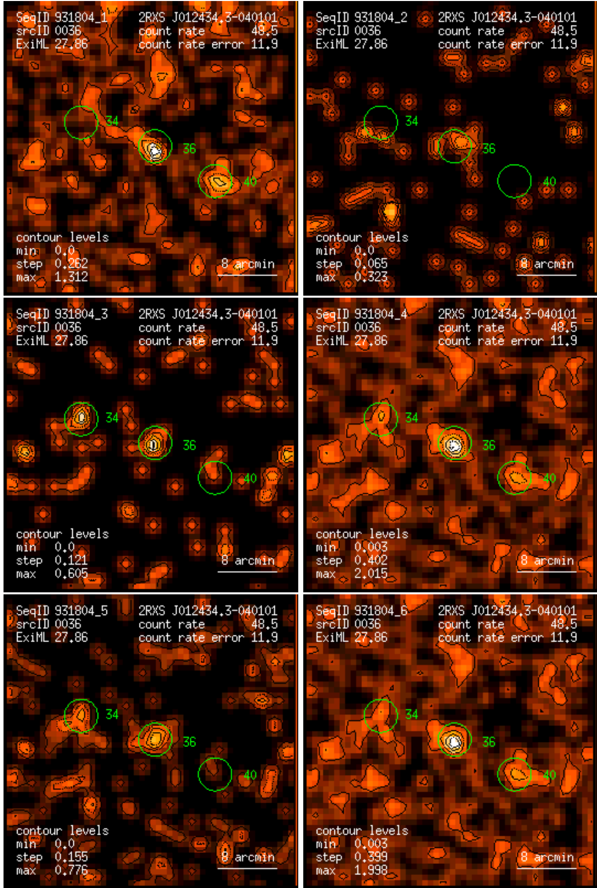
Figure 36: RASS 931804: detection 0036: band rate images, Gaussian filter: (1) PSPC channels 11 – 41, (2) 52 – 90, (3) 91 – 201, (4) 11 – 235, (5) 52 – 201, (6) 11 – 201. Broad band rates in counts/ks. Band rate contour levels in counts/ks/arcmin 2 .
