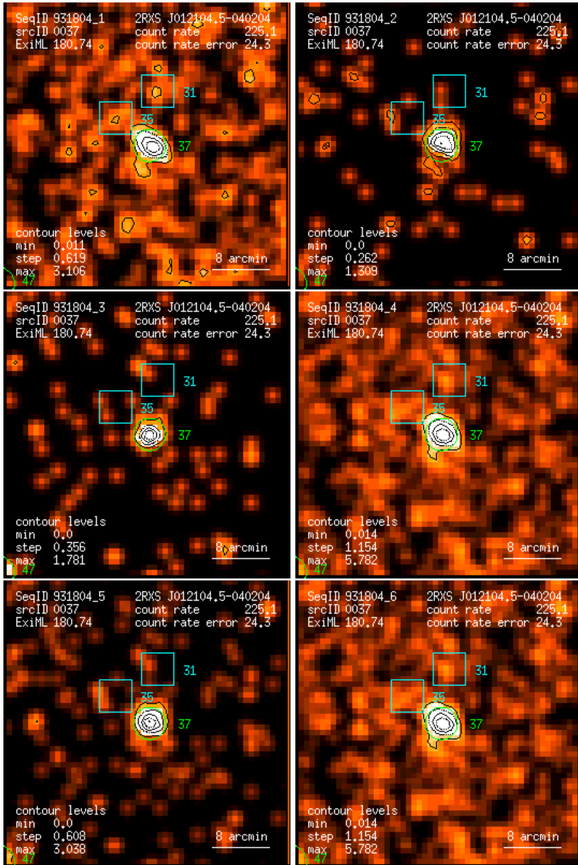
Figure 37: RASS 931804: detection 0037: band rate images, Gaussian filter: (1) PSPC channels 11 – 41, (2) 52 – 90, (3) 91 – 201, (4) 11 – 235, (5) 52 – 201, (6) 11 – 201. Broad band rates in counts/ks. Band rate contour levels in counts/ks/arcmin 2 .
