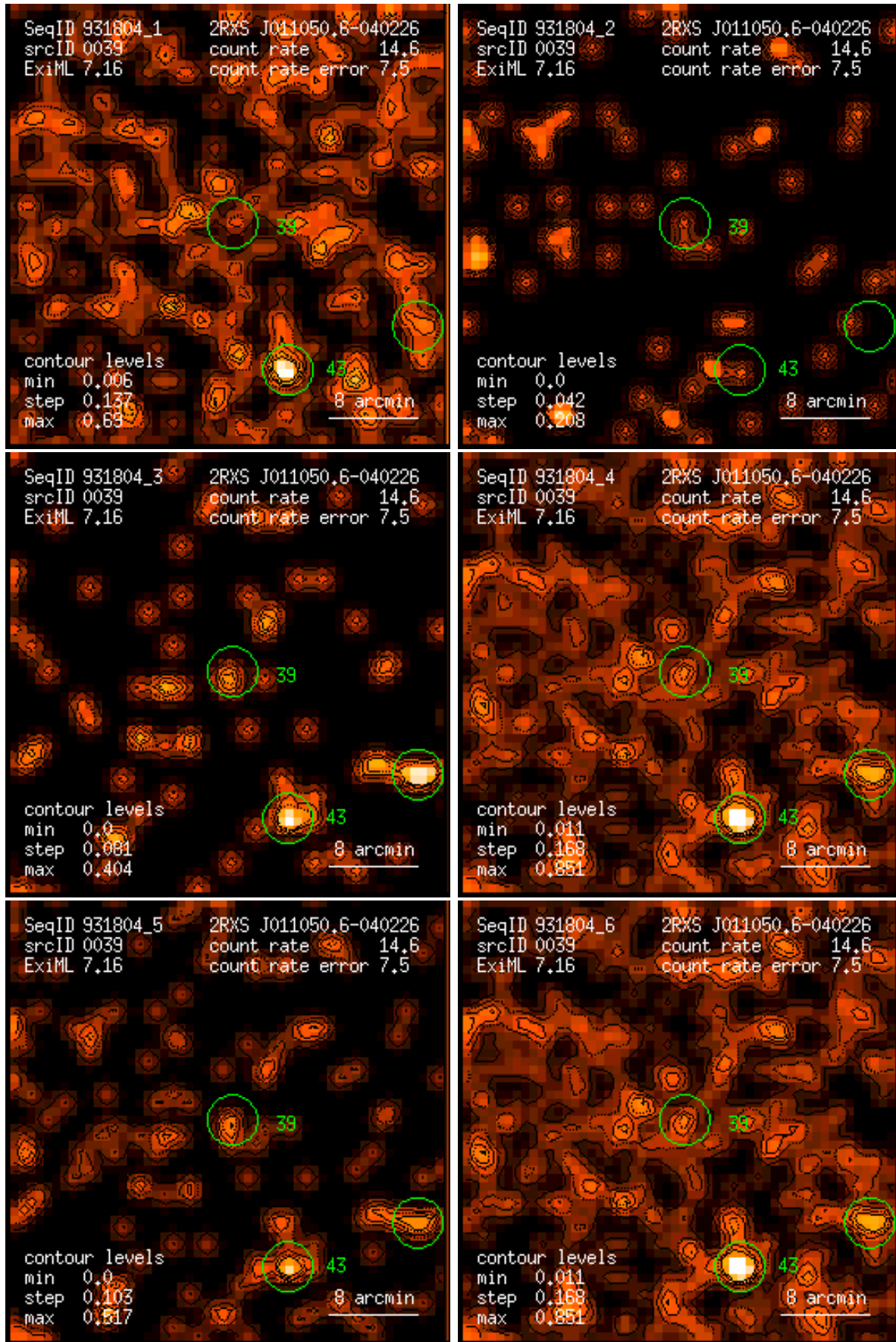
Figure 39: RASS 931804: detection 0039: band rate images, Gaussian filter: (1) PSPC channels 11 – 41, (2) 52 – 90, (3) 91 – 201, (4) 11 – 235, (5) 52 – 201, (6) 11 – 201. Broad band rates in counts/ks. Band rate contour levels in counts/ks/arcmin 2 .
