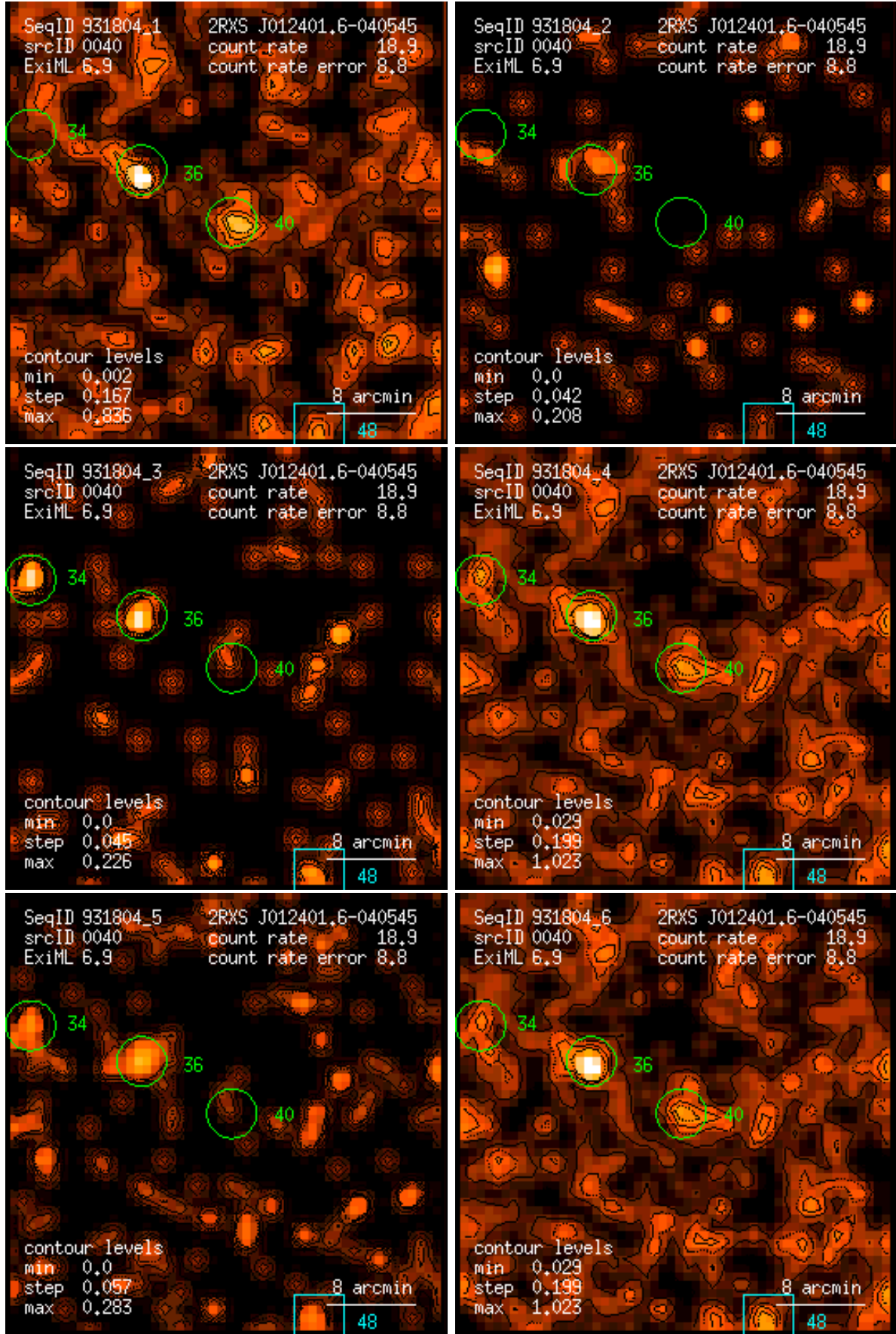
Figure 40: RASS 931804: detection 0040: band rate images, Gaussian filter: (1) PSPPC channels 11 – 41, (2) 52 – 90, (3) 91 – 201, (4) 11 – 235, (5) 52 – 201, (6) 11 – 201. Broad band rates in counts/ks. Band rate contour levels in counts/ks/arcmin 2 .
