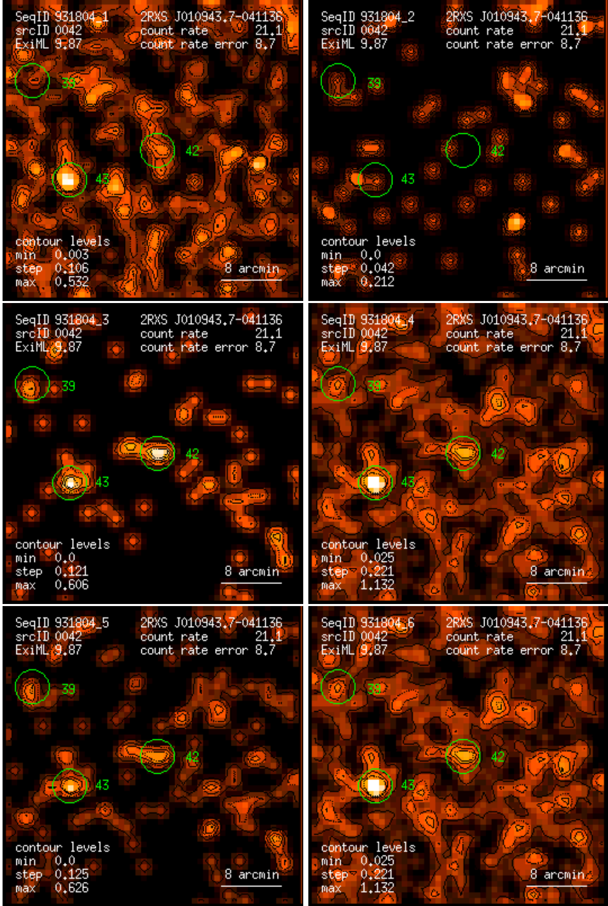
Figure 42: RASS 931804: detection 0042: band rate images, Gaussian filter: (1) PSPC channels 11 – 41, (2) 52 – 90, (3) 91 – 201, (4) 11 – 235, (5) 52 – 201, (6) 11 – 201. Broad band rates in counts/ks. Band rate contour levels in counts/ks/arcmin 2 .
