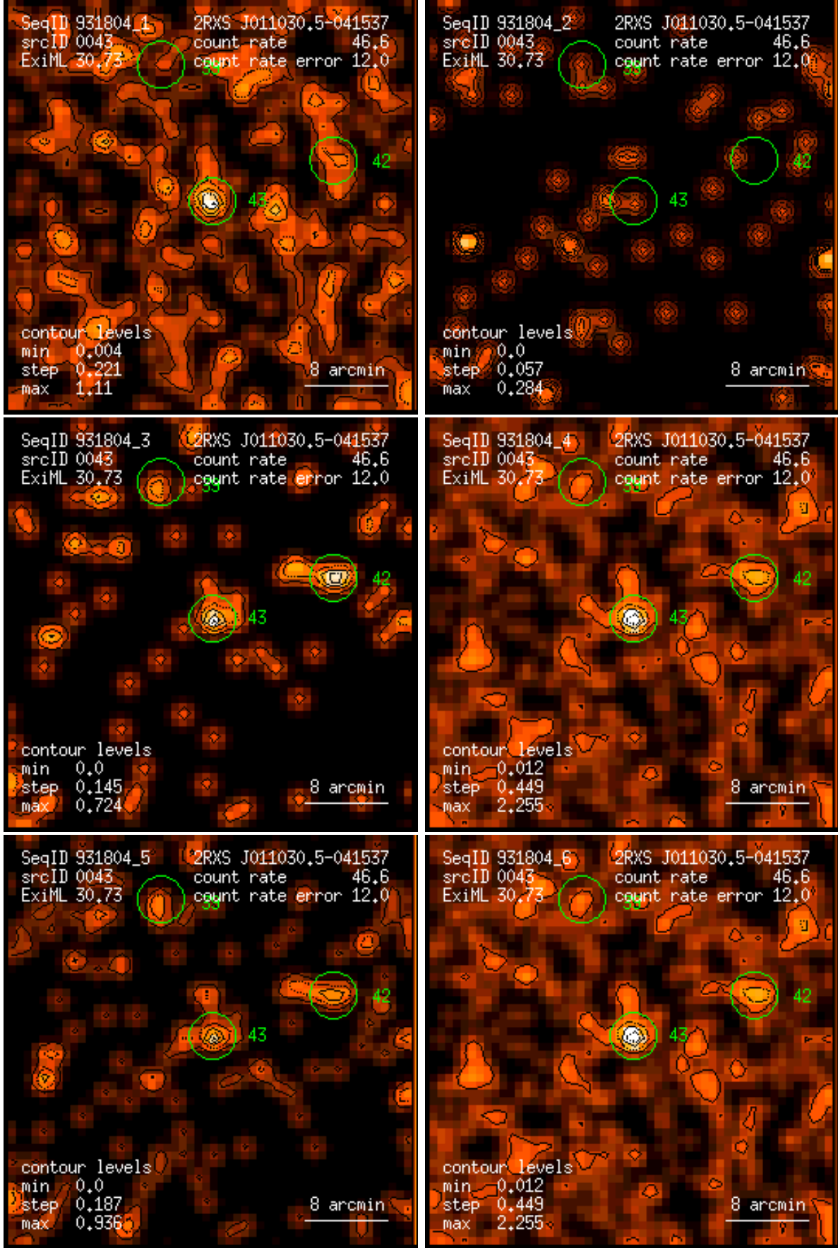
Figure 43: RASS 931804: detection 0043: band rate images, Gaussian filter: (1) PSPC channels 11 – 41, (2) 52 – 90, (3) 91 – 201, (4) 11 – 235, (5) 52 – 201, (6) 11 – 201. Broad band rates in counts/ks. Band rate contour levels in counts/ks/arcmin 2 .
