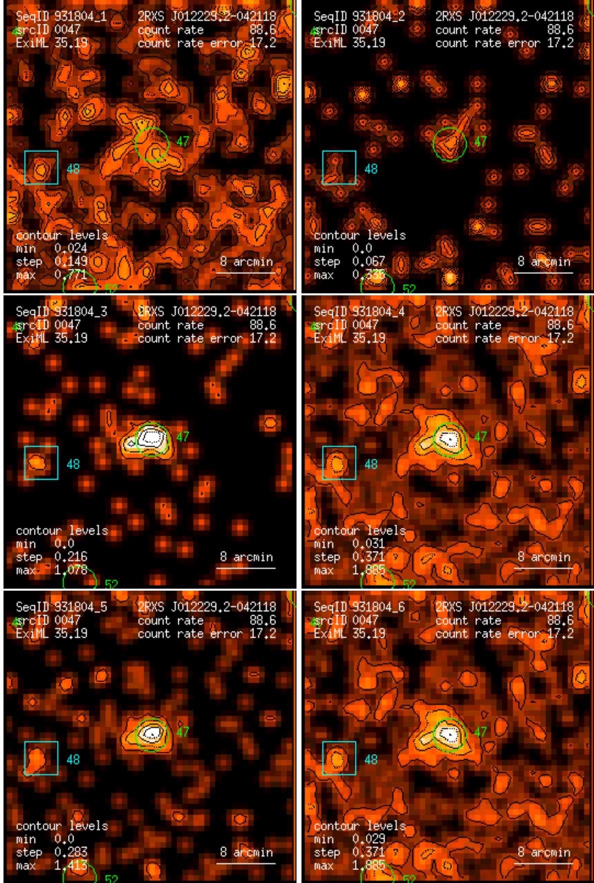
Figure 47: RASS 931804: detection 0047: band rate images, Gaussian filter: (1) PSPC channels 11 – 41, (2) 52 – 90, (3) 91 – 201, (4) 11 – 235, (5) 52 – 201, (6) 11 – 201. Broad band rates in counts/ks. Band rate contour levels in counts/ks/arcmin 2 .
