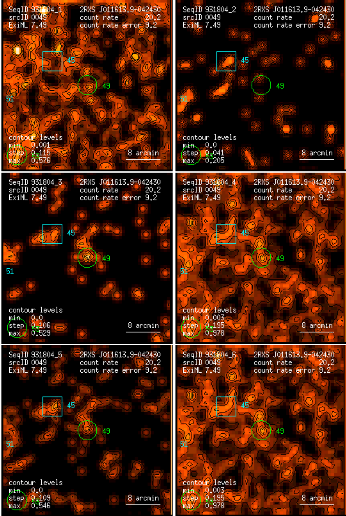
Figure 49: RASS 931804: detection 0049: band rate images, Gaussian filter: (1) PSPC channels 11 – 41, (2) 52 – 90, (3) 91 – 201, (4) 11 – 235, (5) 52 – 201, (6) 11 – 201. Broad band rates in counts/ks. Band rate contour levels in counts/ks/arcmin 2 .
