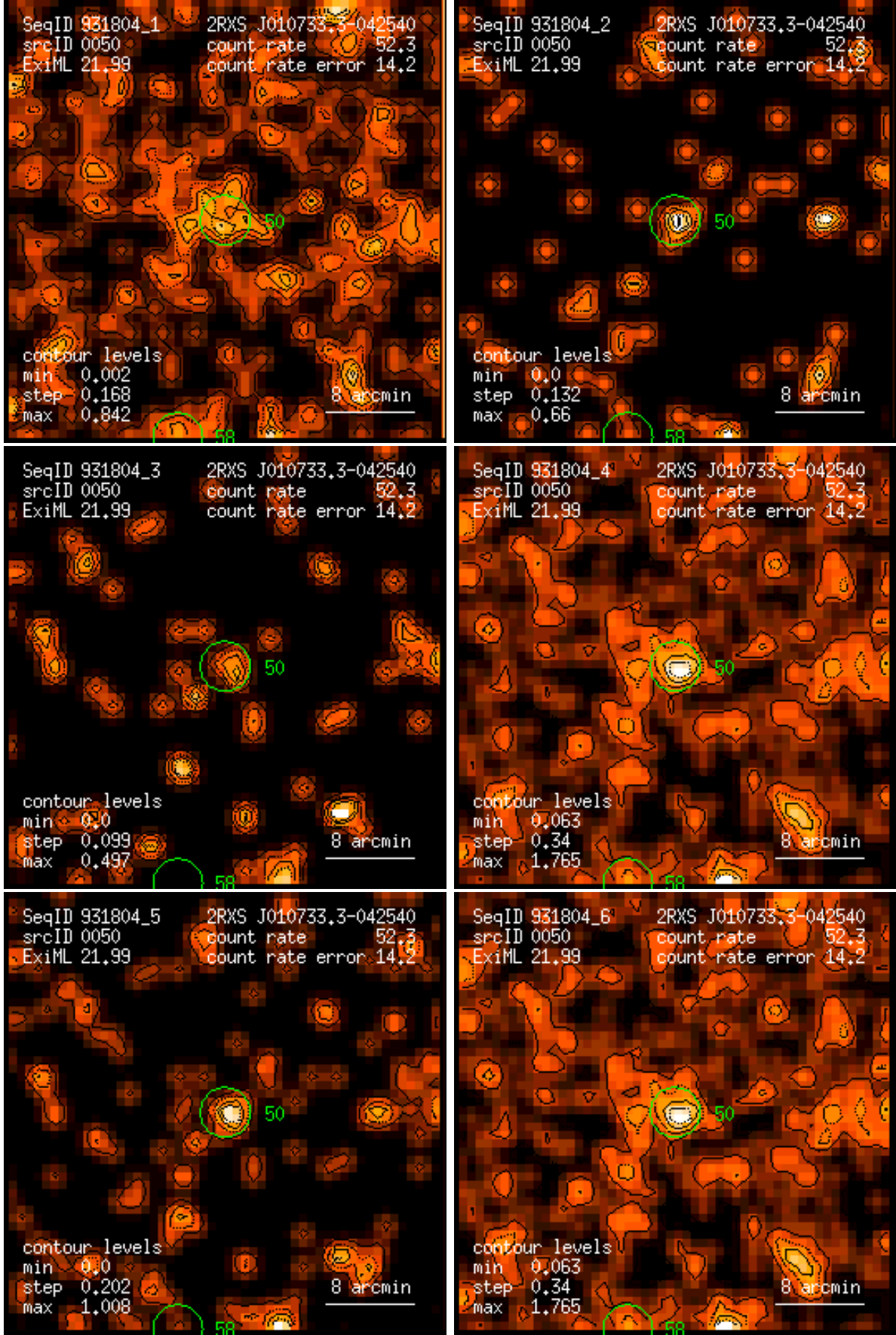
Figure 50: RASS 931804: detection 0050: band rate images, Gaussian filter: (1) PSPC channels 11 – 41, (2) 52 – 90, (3) 91 – 201, (4) 11 – 235, (5) 52 – 201, (6) 11 – 201. Broad band rates in counts/ks. Band rate contour levels in counts/ks/arcmin 2 .
