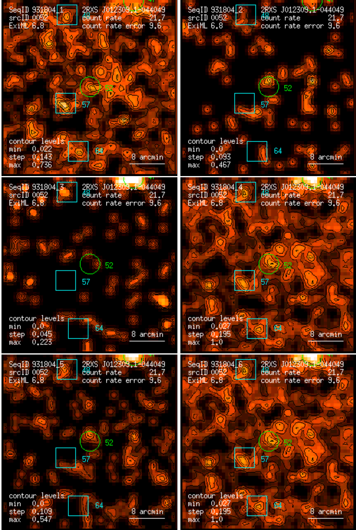
Figure 52: RASS 931804: detection 0052: band rate images, Gaussian filter: (1) PSPC channels 11 – 41, (2) 52 – 90, (3) 91 – 201, (4) 11 – 235, (5) 52 – 201, (6) 11 – 201. Broad band rates in counts/ks. Band rate contour levels in counts/ks/arcmin 2 .
