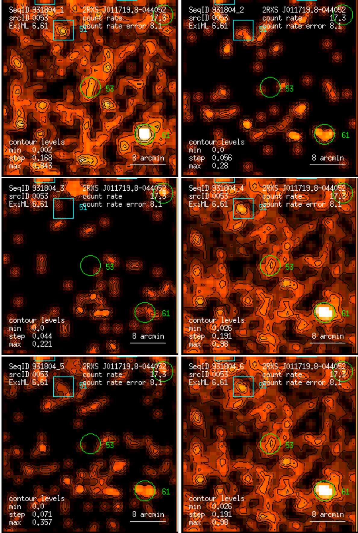
Figure 53: RASS 931804: detection 0053: band rate images, Gaussian filter: (1) PSPC channels 11 – 41, (2) 52 – 90, (3) 91 – 201, (4) 11 – 235, (5) 52 – 201, (6) 11 – 201. Broad band rates in counts/ks. Band rate contour levels in counts/ks/arcmin 2 .
