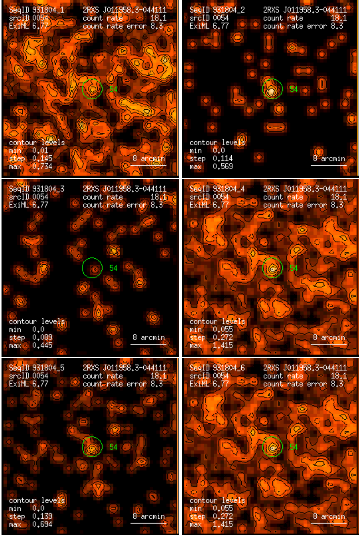
Figure 54: RASS 931804: detection 0054: band rate images, Gaussian filter: (1) PSPC channels 11 – 41, (2) 52 – 90, (3) 91 – 201, (4) 11 – 235, (5) 52 – 201, (6) 11 – 201. Broad band rates in counts/ks. Band rate contour levels in counts/ks/arcmin 2 .
