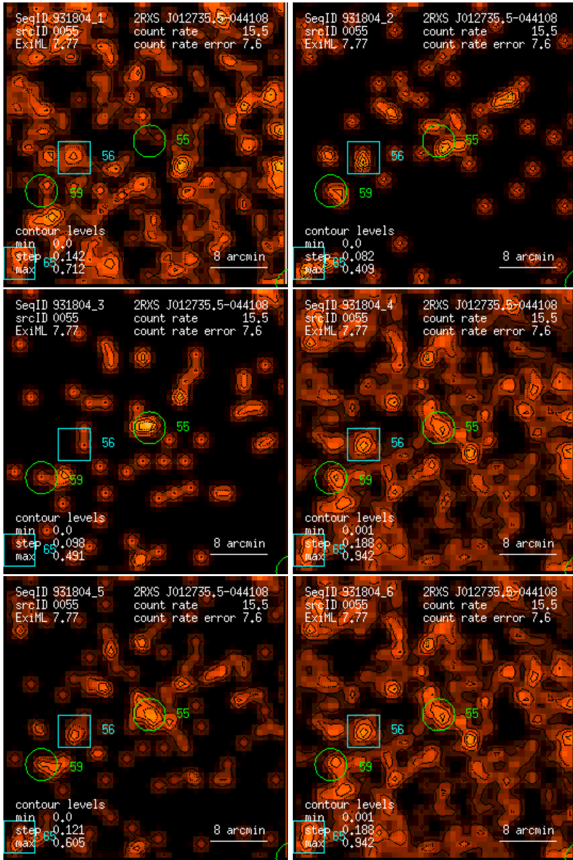
Figure 55: RASS 931804: detection 0055: band rate images, Gaussian filter: (1) PSPC channels 11 – 41, (2) 52 – 90, (3) 91 – 201, (4) 11 – 235, (5) 52 – 201, (6) 11 – 201. Broad band rates in counts/ks. Band rate contour levels in counts/ks/arcmin 2 .
