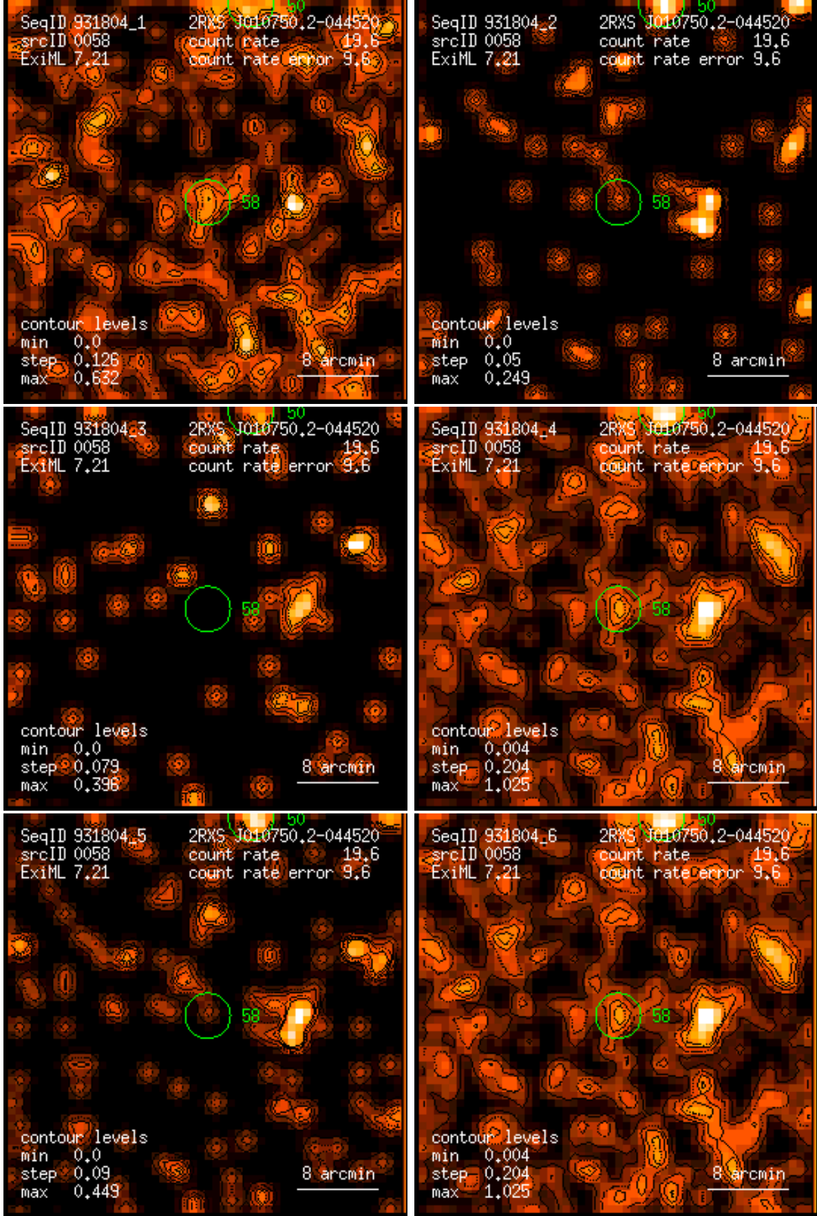
Figure 58: RASS 931804: detection 0058: band rate images, Gaussian filter: (1) PSPC channels 11 – 41, (2) 52 – 90, (3) 91 – 201, (4) 11 – 235, (5) 52 – 201, (6) 11 – 201. Broad band rates in counts/ks. Band rate contour levels in counts/ks/arcmin 2 .
