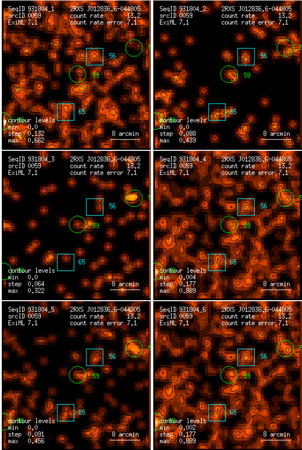
Figure 59: RASS 931804: detection 0059: band rate images, Gaussian filter: (1) PSPC channels 11 – 41, (2) 52 – 90, (3) 91 – 201, (4) 11 – 235, (5) 52 – 201, (6) 11 – 201. Broad band rates in counts/ks. Band rate contour levels in counts/ks/arcmin 2 .
