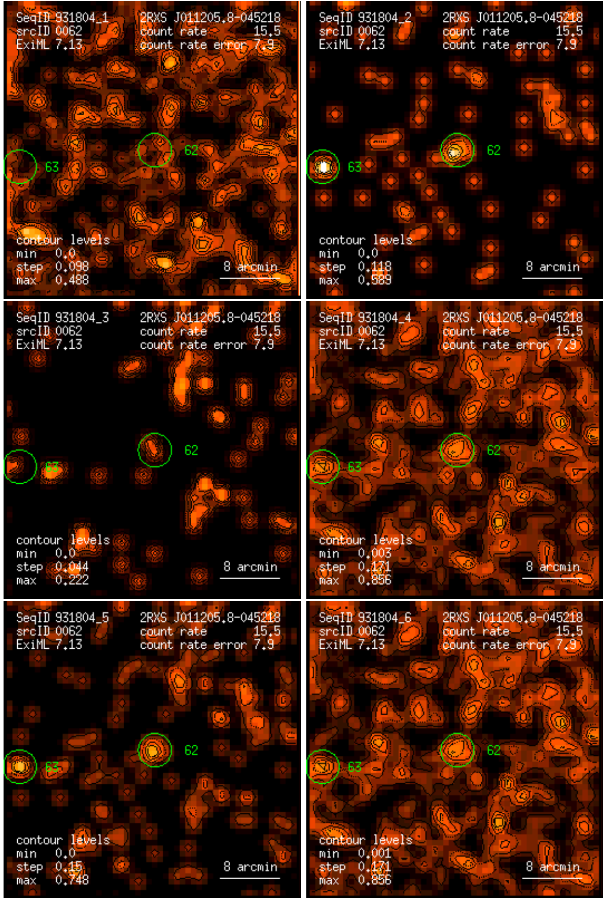
Figure 62: RASS 931804: detection 0062: band rate images, Gaussian filter: (1) PSPC channels 11 – 41, (2) 52 – 90, (3) 91 – 201, (4) 11 – 235, (5) 52 – 201, (6) 11 – 201. Broad band rates in counts/ks. Band rate contour levels in counts/ks/arcmin 2 .
