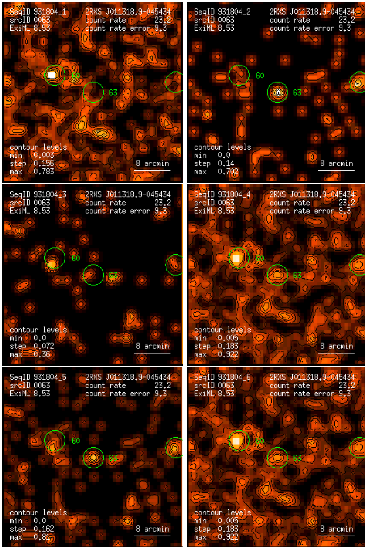
Figure 63: RASS 931804: detection 0063: band rate images, Gaussian filter: (1) PSPC channels 11 – 41, (2) 52 – 90, (3) 91 – 201, (4) 11 – 235, (5) 52 – 201, (6) 11 – 201. Broad band rates in counts/ks. Band rate contour levels in counts/ks/arcmin 2 .
