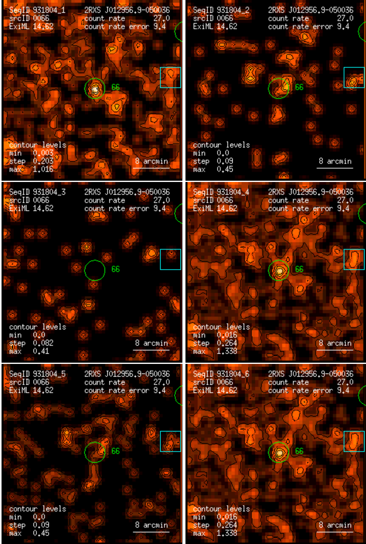
Figure 66: RASS 931804: detection 0066: band rate images, Gaussian filter: (1) PSPC channels 11 – 41, (2) 52 – 90, (3) 91 – 201, (4) 11 – 235, (5) 52 – 201, (6) 11 – 201. Broad band rates in counts/ks. Band rate contour levels in counts/ks/arcmin 2 .
