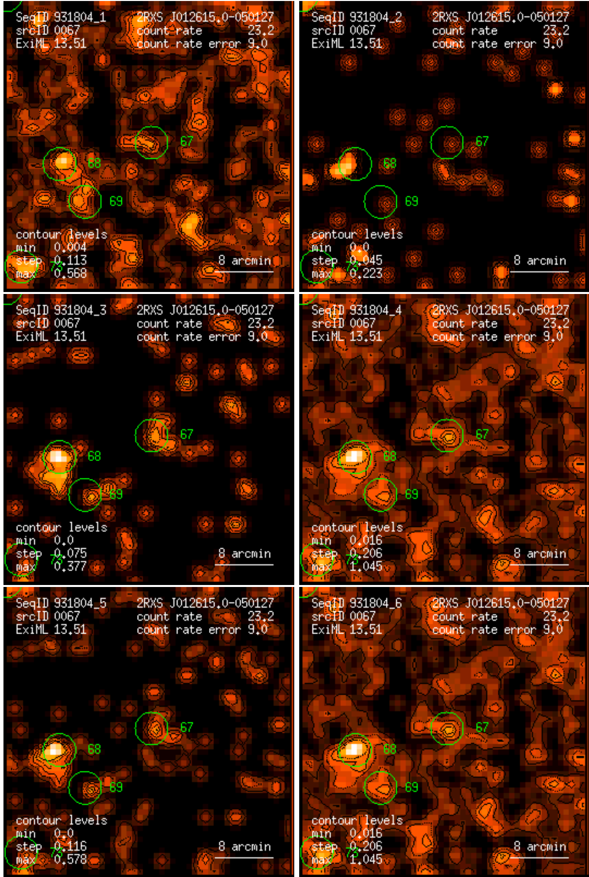
Figure 67: RASS 931804: detection 0067: band rate images, Gaussian filter: (1) PSPC channels 11 – 41, (2) 52 – 90, (3) 91 – 201, (4) 11 – 235, (5) 52 – 201, (6) 11 – 201. Broad band rates in counts/ks. Band rate contour levels in counts/ks/arcmin 2 .
