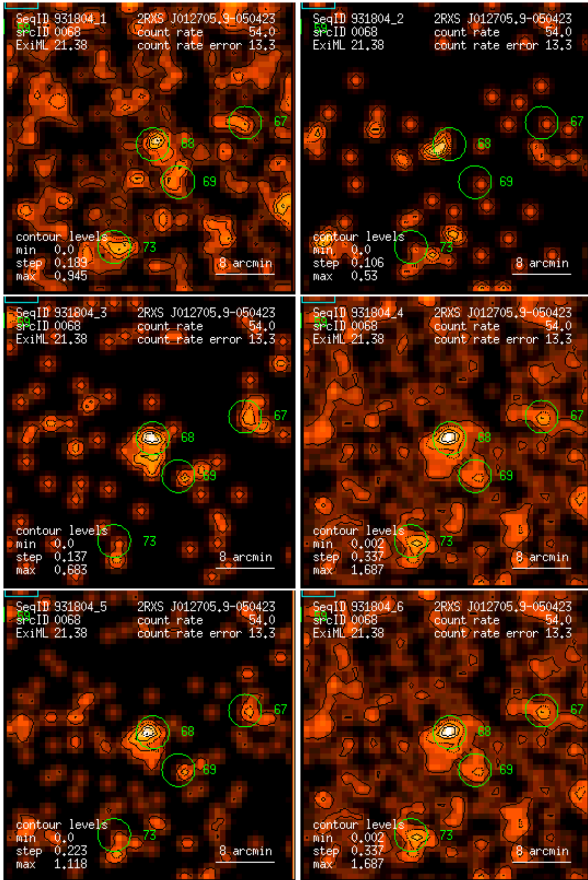
Figure 68: RASS 931804: detection 0068: band rate images, Gaussian filter: (1) PSPC channels 11 – 41, (2) 52 – 90, (3) 91 – 201, (4) 11 – 235, (5) 52 – 201, (6) 11 – 201. Broad band rates in counts/ks. Band rate contour levels in counts/ks/arcmin 2 .
