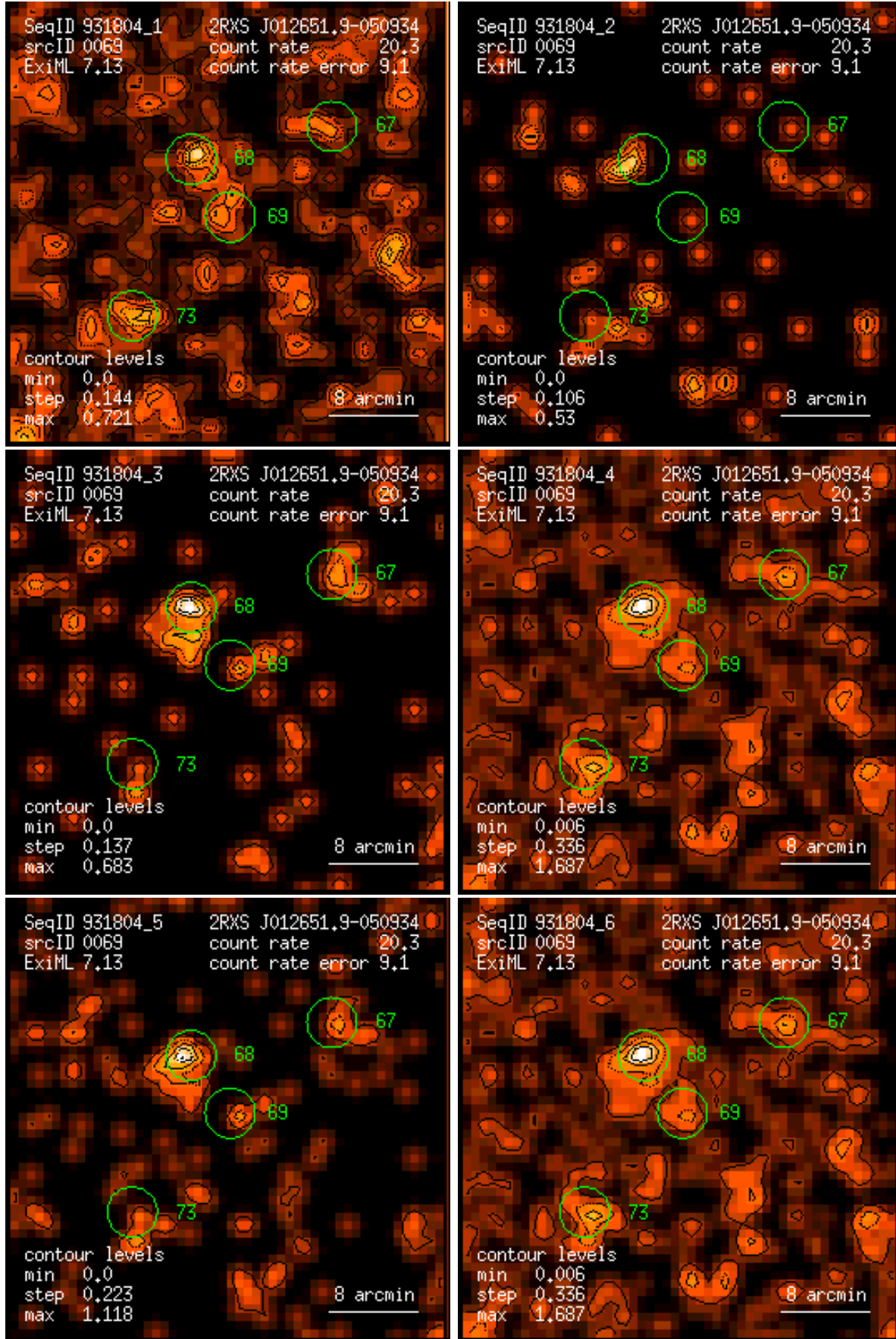
Figure 69: RASS 931804: detection 0069: band rate images, Gaussian filter: (1) PSPC channels 11 – 41, (2) 52 – 90, (3) 91 – 201, (4) 11 – 235, (5) 52 – 201, (6) 11 – 201. Broad band rates in counts/ks. Band rate contour levels in counts/ks/arcmin 2 .
